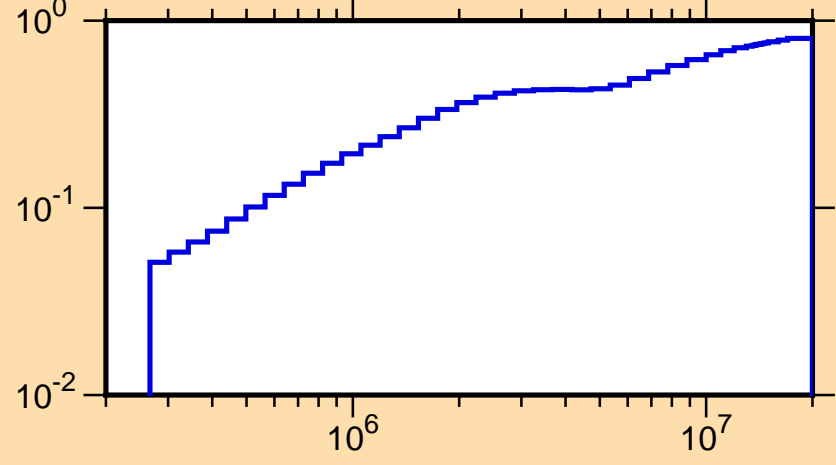
\mu vs. E for ^{22}\text{Ne}(\text{mt251})
