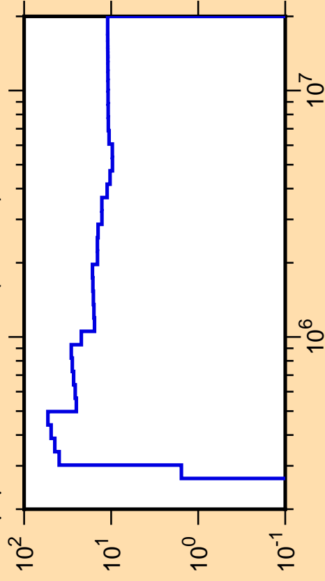
\Delta\mu/\mu vs. E for ^{22}\text{Ne}(\text{mt251})
