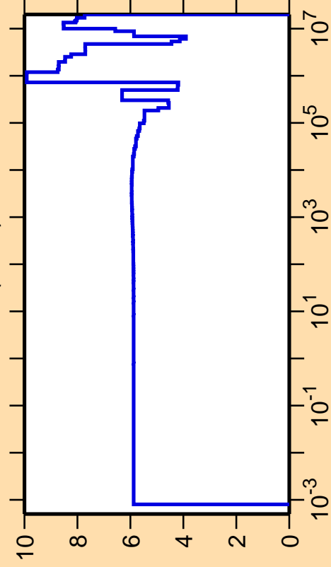
\Delta\sigma/\sigma vs. E for ^{22}\text{Ne}(n,\text{el.})
