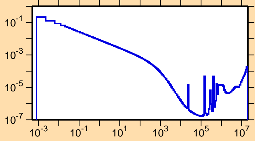
\sigma vs. E for ^{22}\text{Ne}(n,\gamma)
