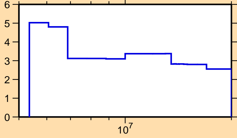
\Delta\sigma/\sigma vs. E for ^{22}\text{Ne}(n,\text{tot.})
