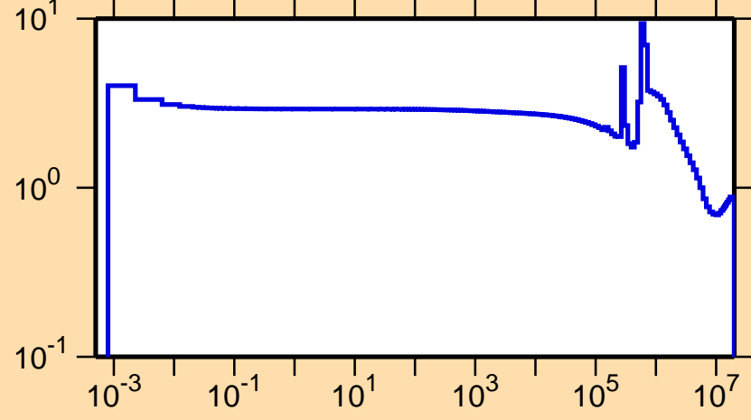
\sigma vs. E for ^{22}\text{Ne}(n,\text{el.})
