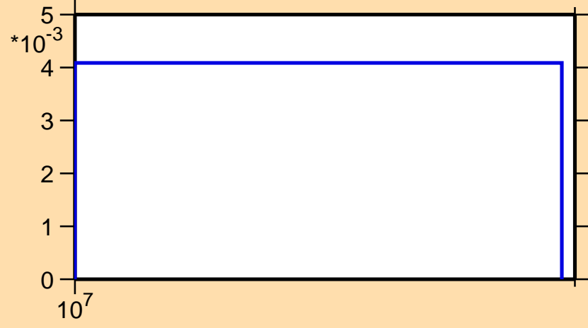
\sigma vs. E for ^{22}\text{Ne}(n,p)
