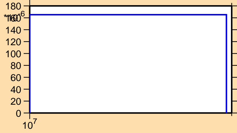
\sigma vs. E for ^{22}\text{Ne}(n,d)
