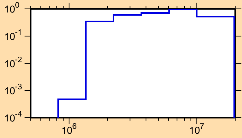
\sigma vs. E for ^{22}\text{Ne}(n,\text{inel.})
