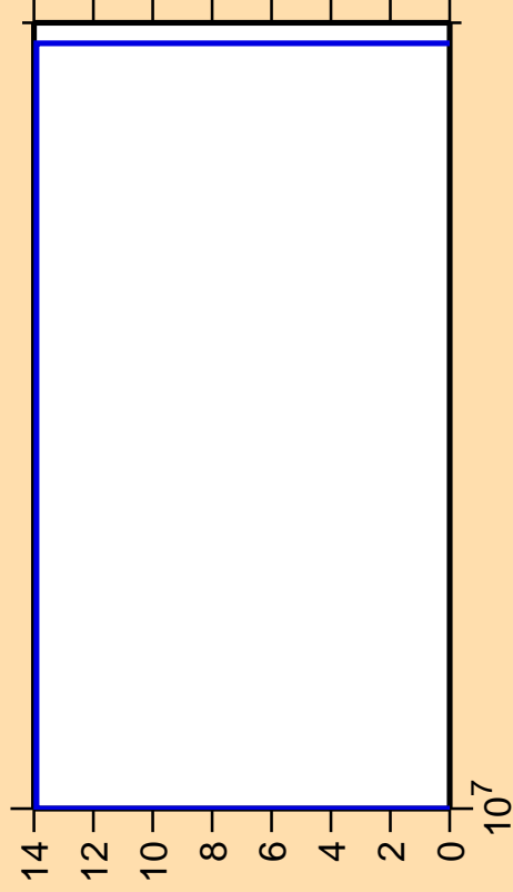
\Delta\sigma/\sigma vs. E for ^{22}\text{Ne}(n,ncont.)
