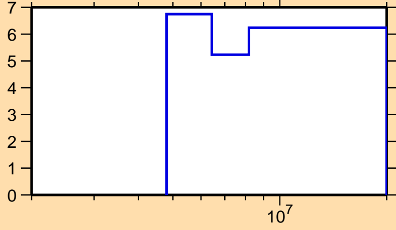
\Delta\sigma/\sigma vs. E for ^{22}\text{Ne}(n,\text{nonel.})
