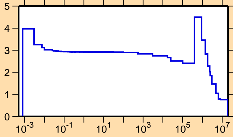
\sigma vs. E for ^{22}\text{Ne}(n,\text{el.})
