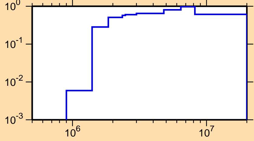
\sigma vs. E for ^{22}\text{Ne}(n,\text{inel.})
