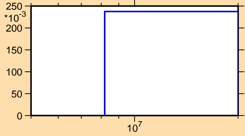
\sigma vs. E for ^{22}\text{Ne}(n,n\text{cont.})
