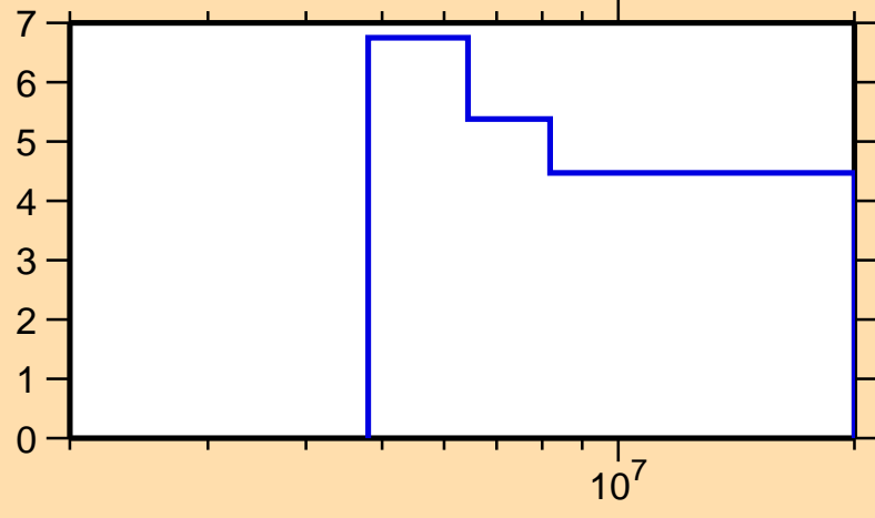
\Delta\sigma/\sigma vs. E for ^{22}\text{Ne}(n,\text{inel.})
