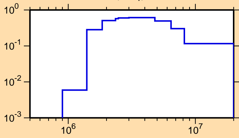
\sigma vs. E for ^{22}\text{Ne}(n,n_1)
