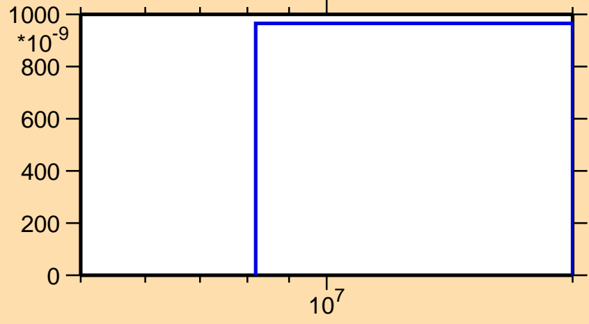
\sigma vs. E for ^{22}\text{Ne}(n,3n)
