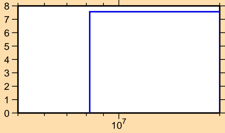
\Delta\sigma/\sigma vs. E for ^{22}\text{Ne}(n,el.)
