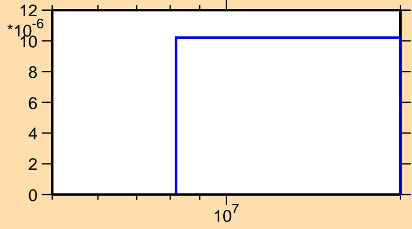
\sigma vs. E for ^{22}\text{Ne}(n,np)
