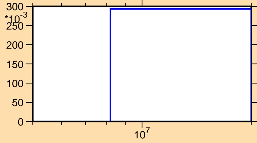
\sigma vs. E for ^{22}\text{Ne}(n,2n)
