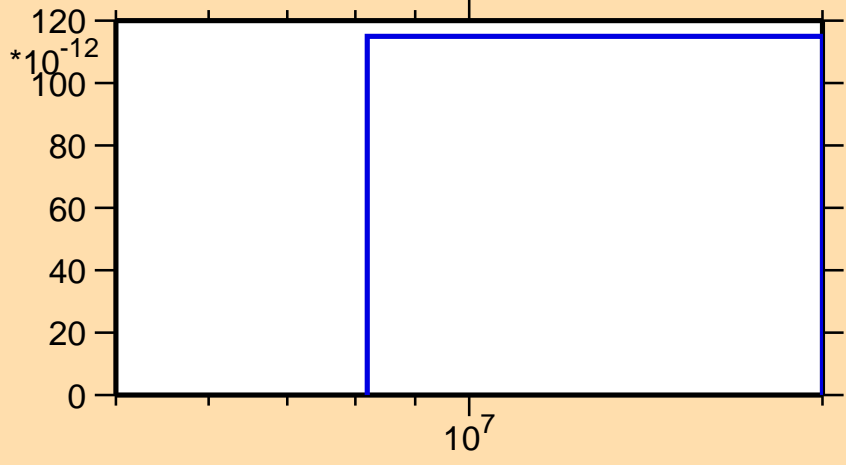
\sigma vs. E for ^{22}\text{Ne}(n,2n\alpha)
