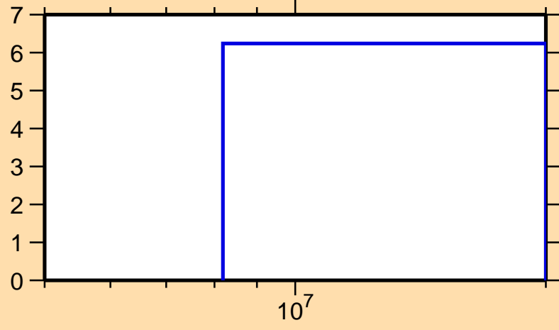
\Delta\sigma/\sigma vs. E for ^{22}\text{Ne}(n,n\text{onel.})
