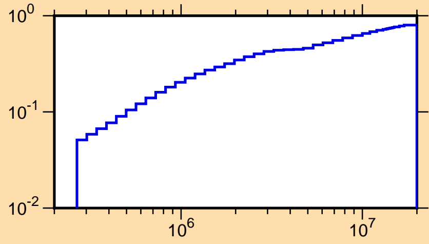
\mu vs. E for ^{23}\text{Ne}(\text{mt251})
