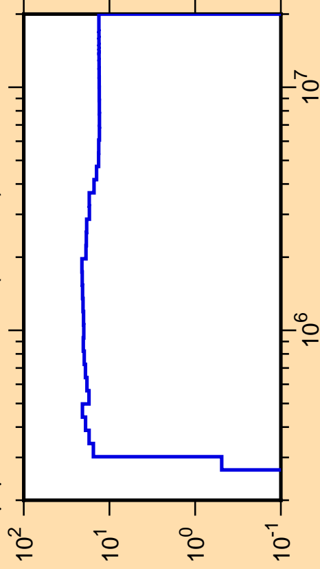
\Delta\mu/\mu vs. E for ^{23}\text{Ne}(\text{mt251})
