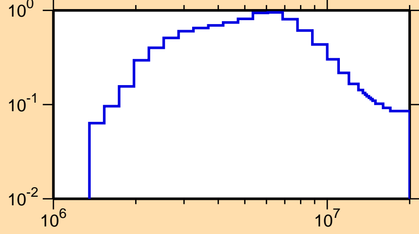
\sigma vs. E for ^{23}\text{Ne}(n,\text{inel.})
