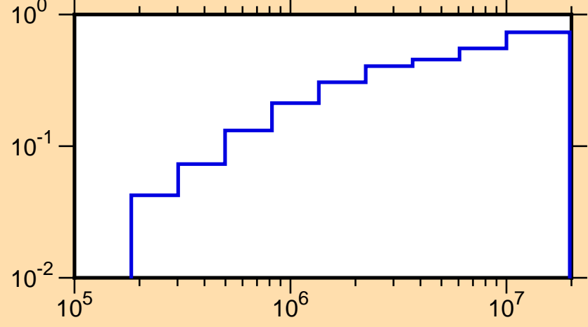
\mu vs. E for ^{23}\text{Ne}(\text{mt251})
