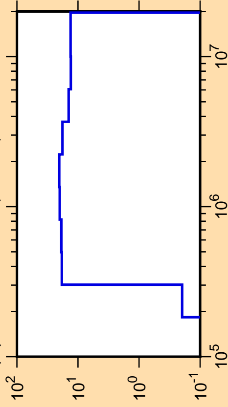
\Delta\mu/\mu vs. E for ^{23}\text{Ne}(\text{mt251})
