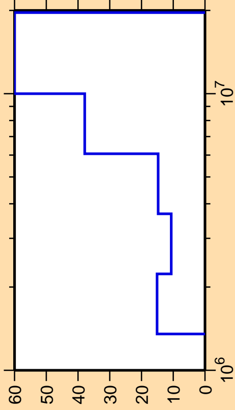
\Delta\sigma/\sigma vs. E for ^{23}\text{Ne}(n,n_2)
