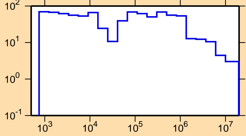
\Delta\sigma/\sigma vs. E for ^{23}\text{Ne}(n,\text{tot.})
