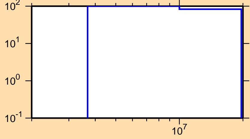
\Delta\sigma/\sigma vs. E for ^{23}\text{Ne}(n,n\text{cont.})
