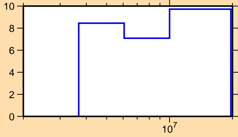
\Delta\sigma/\sigma vs. E for ^{23}\text{Ne}(n,n\text{inel.})
