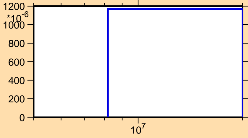
\sigma vs. E for ^{23}\text{Ne}(n,\alpha)
