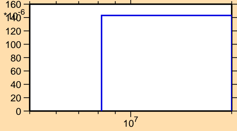
\sigma vs. E for ^{23}\text{Ne}(n,t)
