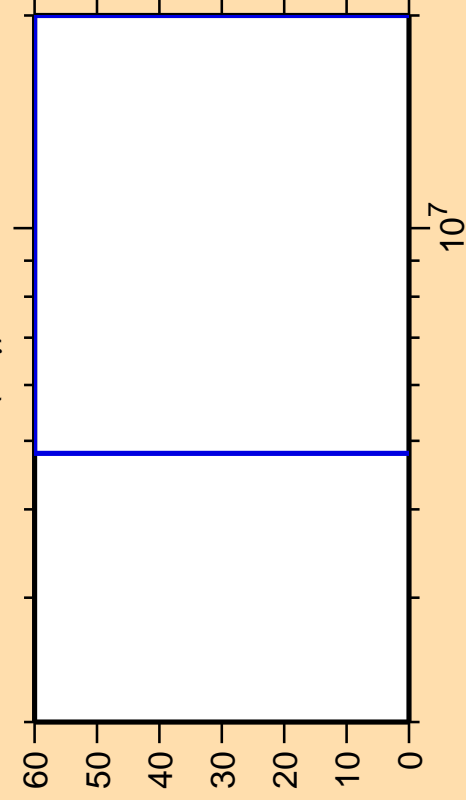
\Delta\sigma/\sigma vs. E for ^{23}\text{Ne}(n,\gamma)
