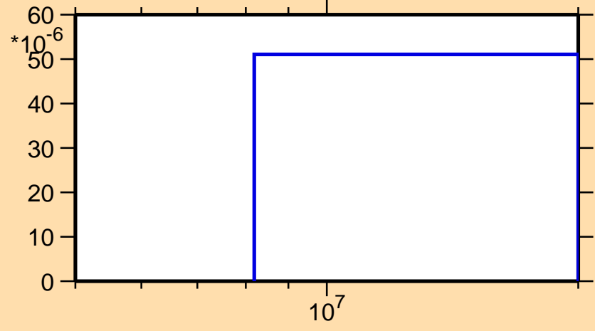
\sigma vs. E for ^{23}\text{Ne}(n,3n)
