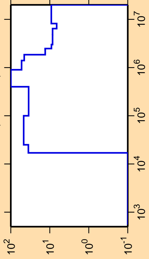
\Delta\sigma/\sigma vs. E for ^{23}\text{Ne}(n,\text{nonel.})
