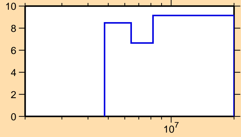
\Delta\sigma/\sigma vs. E for ^{23}\text{Ne}(n,n\text{onel.})
