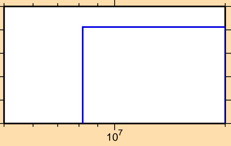
\sigma vs. E for ^{23}\text{Ne}(n,d)
