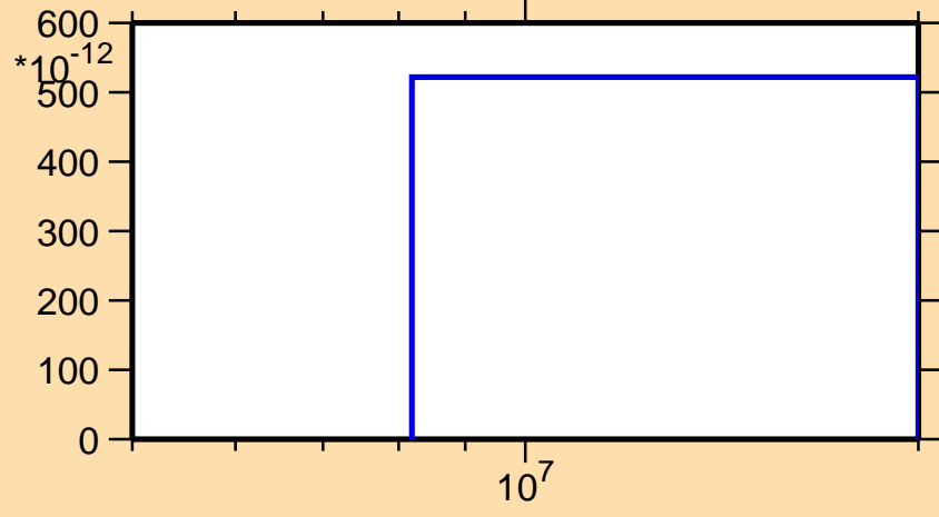
\sigma vs. E for ^{23}\text{Ne}(n,\text{nd})
