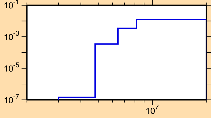
\sigma vs. E for ^{23}\text{Ne}(n,\alpha)
