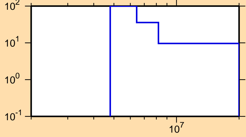
\Delta\sigma/\sigma vs. E for ^{23}\text{Ne}(n,2n)
