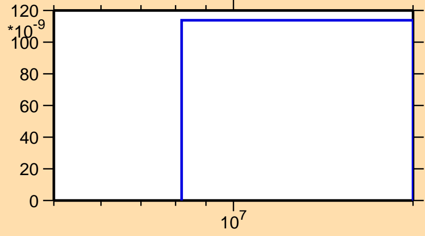
\sigma vs. E for ^{23}\text{Ne}(n,2n\alpha)
