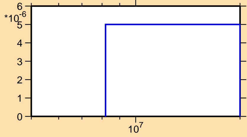
\sigma vs. E for ^{23}\text{Ne}(n,np)
