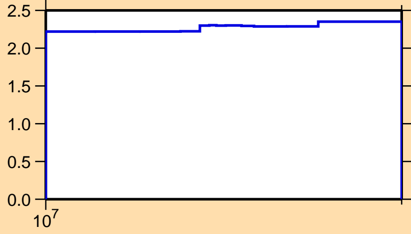
\Delta\sigma/\sigma vs. E for ^{24}\text{Ne}(n,n\text{onel.})
