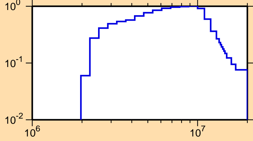
\sigma vs. E for ^{24}\text{Ne}(n,\text{inel.})
