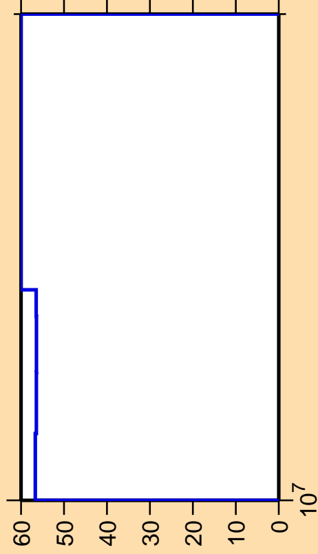
\Delta\sigma/\sigma vs. E for ^{24}\text{Ne}(n,ncont.)
