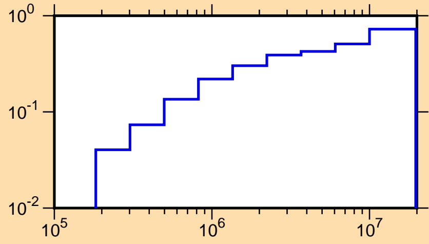
\mu vs. E for ^{24}\text{Ne}(\text{mt251})
