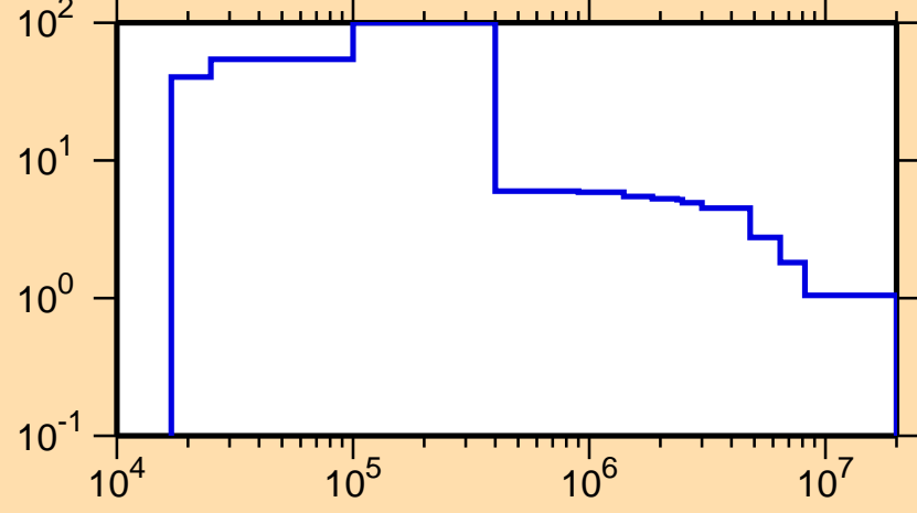
\Delta\sigma/\sigma vs. E for ^{24}\text{Ne}(n,\text{tot.})
