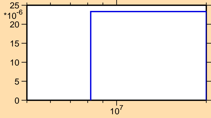
\sigma vs. E for ^{24}\text{Ne}(n,n\text{cont.})
