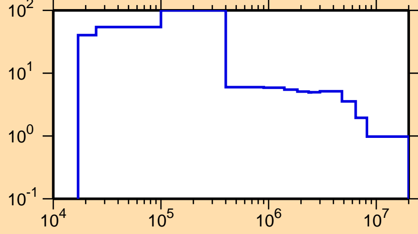
\Delta\sigma/\sigma vs. E for ^{24}\text{Ne}(n,\text{el.})
