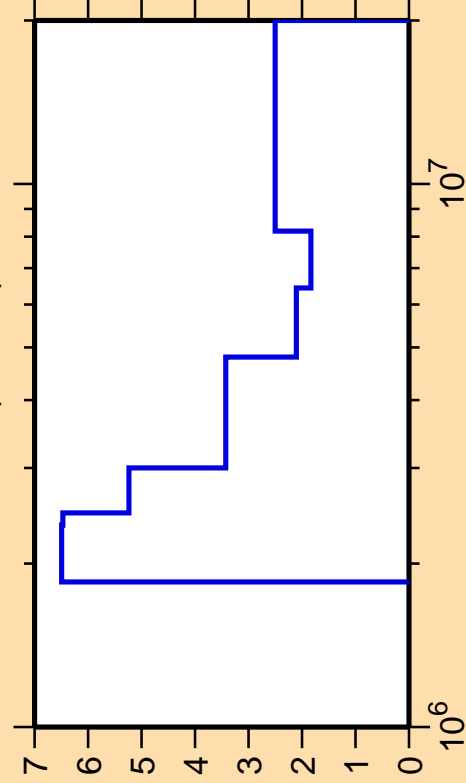
\Delta\sigma/\sigma vs. E for ^{24}\text{Ne}(n,\text{inel.})
