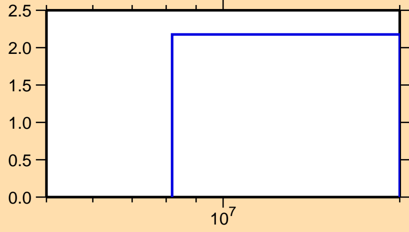
\Delta\sigma/\sigma vs. E for ^{24}\text{Ne}(n,n\text{nonel.})
