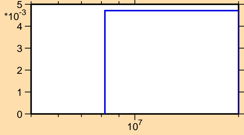
\sigma vs. E for ^{24}\text{Ne}(n,\alpha)
