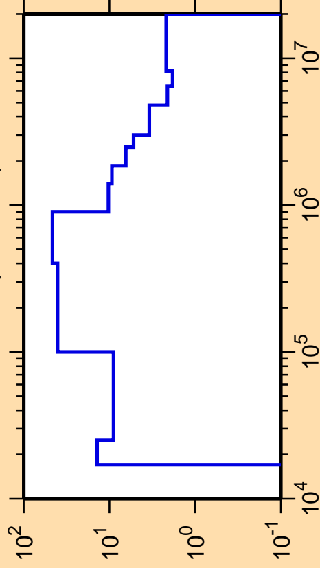
\Delta\sigma/\sigma vs. E for ^{24}\text{Ne}(n,\text{nonel.})
