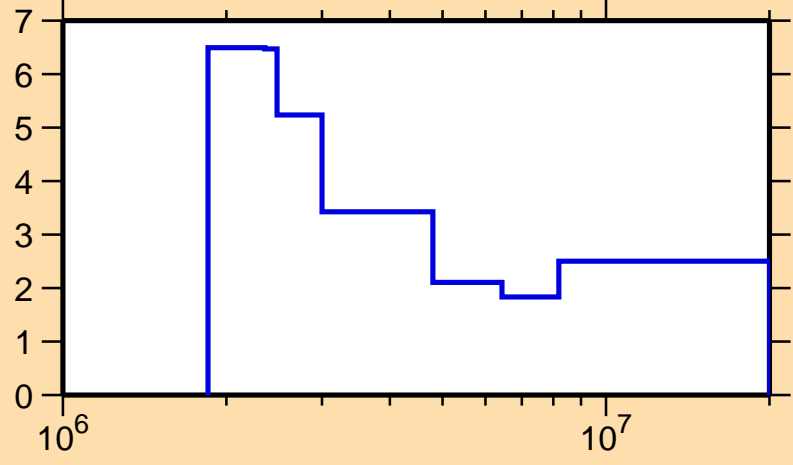
\Delta\sigma/\sigma vs. E for ^{24}\text{Ne}(n,\text{inel.})
