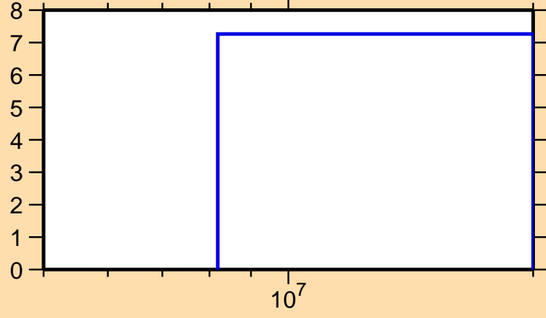
\Delta\sigma/\sigma vs. E for ^{24}\text{Ne}(n,n_1)
