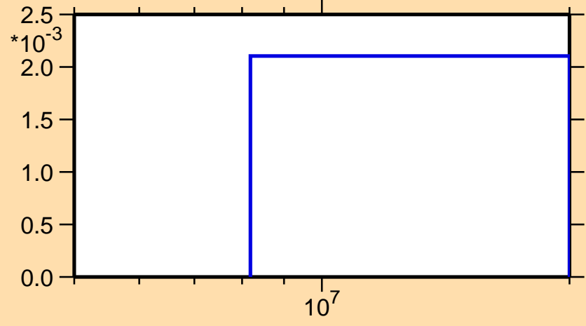
\sigma vs. E for ^{24}\text{Ne}(n,3n)
