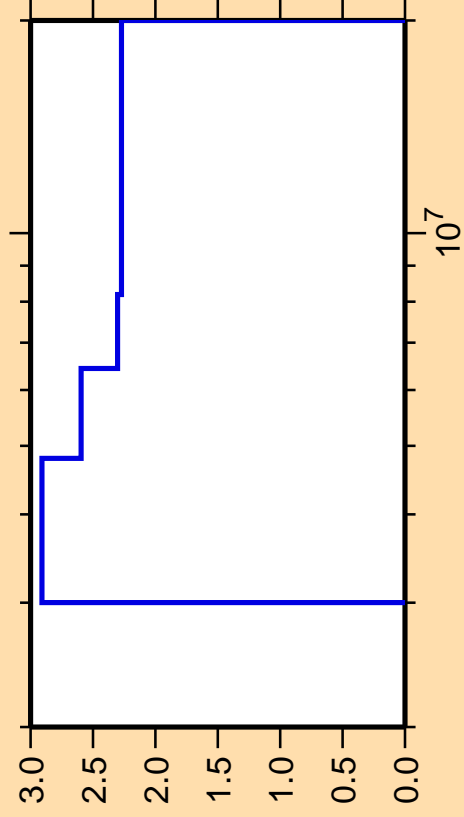
\Delta\sigma/\sigma vs. E for ^{24}\text{Ne}(n,n_3)
