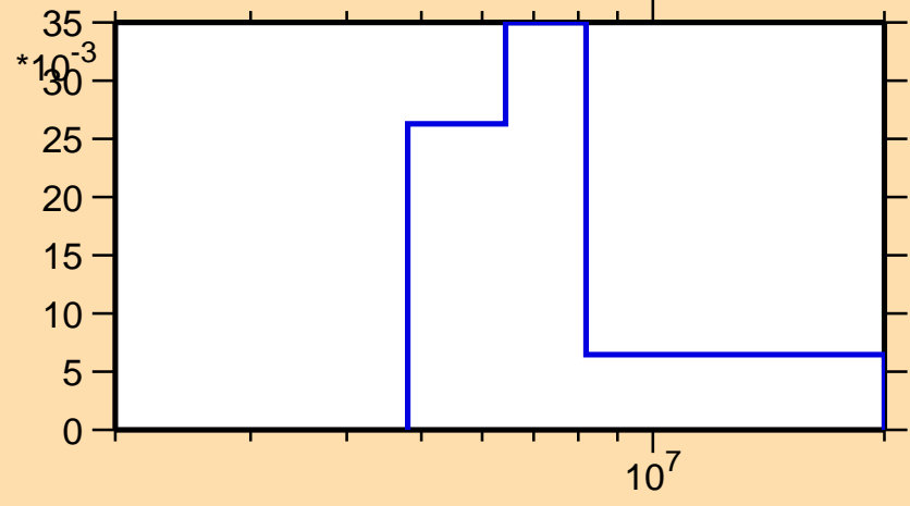
\sigma vs. E for ^{24}\text{Ne}(n,n_4)
