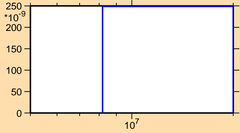
\sigma vs. E for ^{24}\text{Ne}(n,np)
