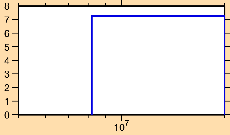
\Delta\sigma/\sigma vs. E for ^{24}\text{Ne}(n,n_1)
