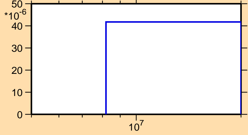
\sigma vs. E for ^{24}\text{Ne}(n,d)
