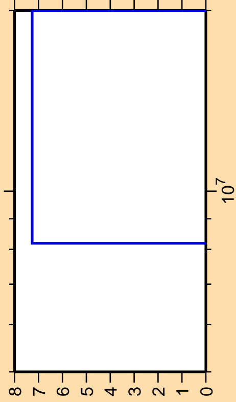
\Delta\sigma/\sigma vs. E for ^{24}\text{Ne}(n,n_1)
