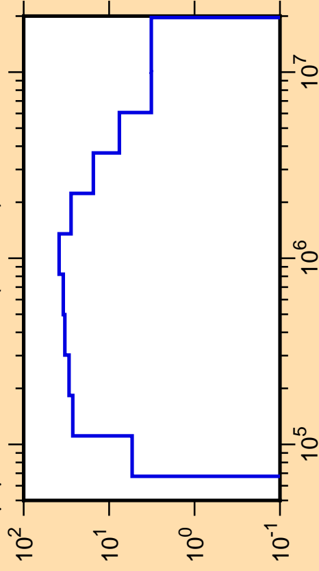
\Delta\mu/\mu vs. E for ^{56}\text{Ni}(\text{mt251})
