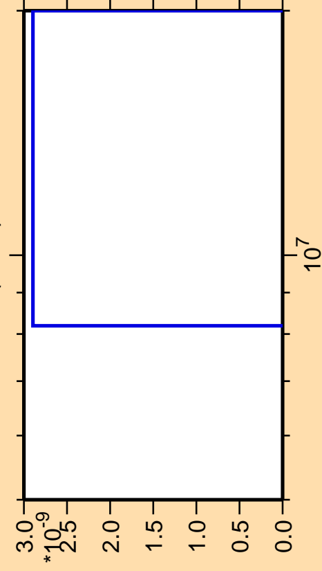
\Delta\sigma/\sigma vs. E for ^{56}\text{Ni}(n,\text{nd})
