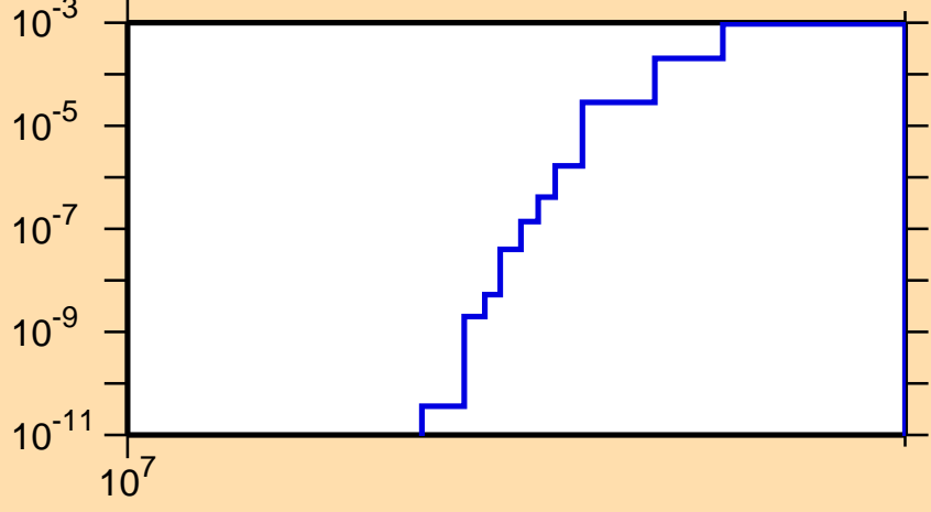
\sigma vs. E for ^{57}\text{Ni}(n,\text{pd})
