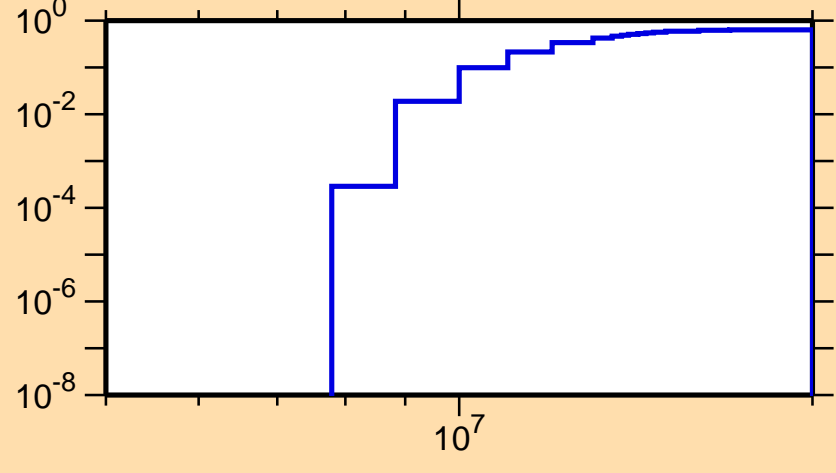
\sigma vs. E for ^{57}\text{Ni}(n,np)
