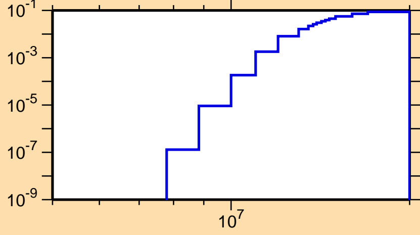
\sigma vs. E for ^{57}\text{Ni}(n,p\alpha)
