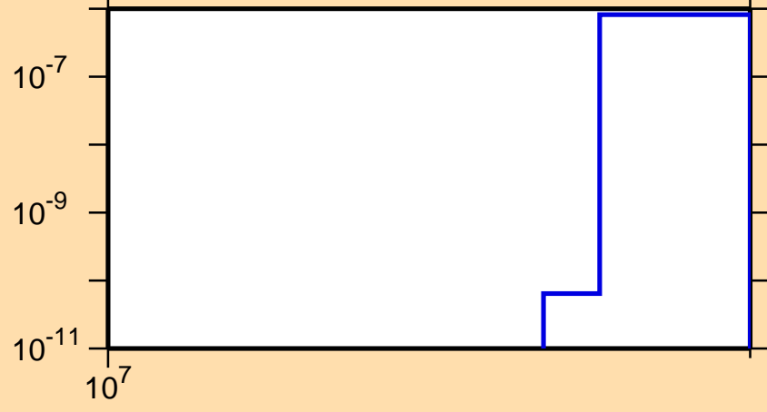
\sigma vs. E for ^{57}\text{Ni}(n,\text{pt})
