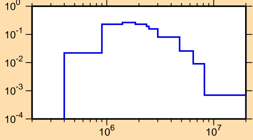
\sigma vs. E for ^{57}\text{Ni}(n,n_1)
