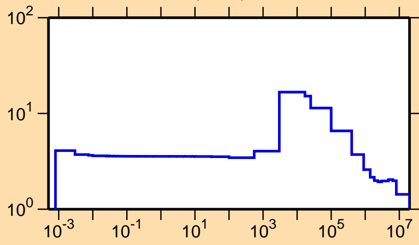
\sigma vs. E for ^{57}\text{Ni}(n,\text{el.})
