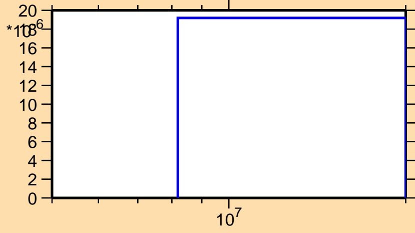
\sigma vs. E for ^{57}\text{Ni}(n,pd)
