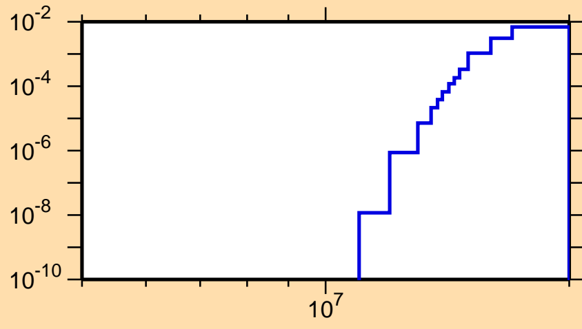
\sigma vs. E for ^{58}\text{Ni}(n,p\alpha)
