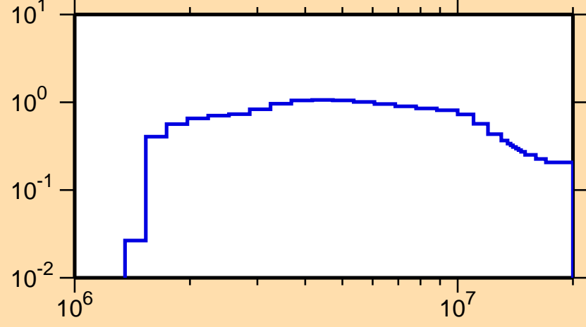
\sigma vs. E for ^{58}\text{Ni}(n,\text{inel.})
