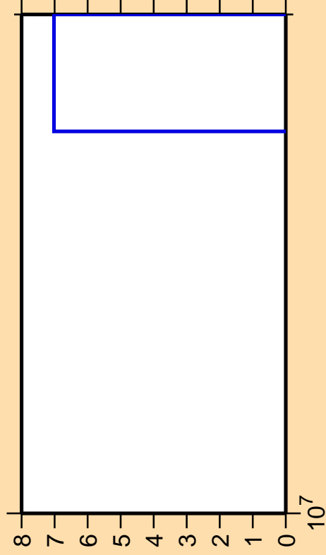
\Delta\sigma/\sigma vs. E for ^{58}\text{Ni}(n,\text{pt})
