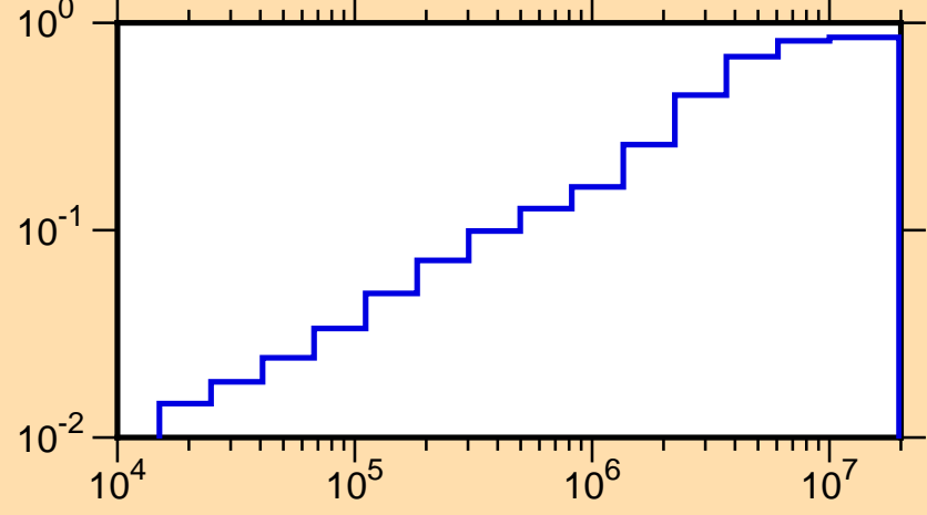
\mu vs. E for ^{58}\text{Ni}(\text{mt251})
