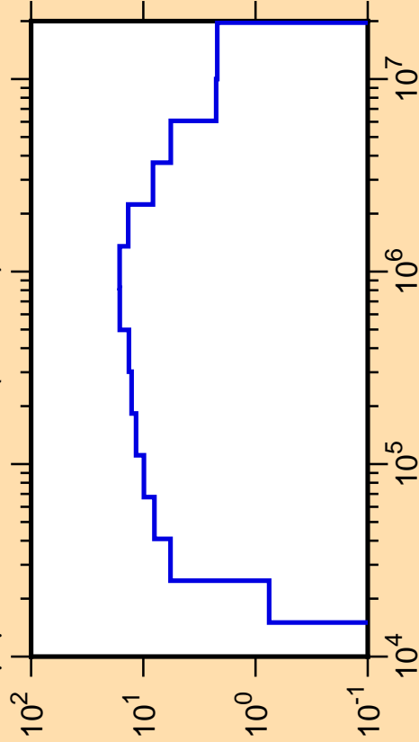
\Delta\mu/\mu vs. E for ^{58}\text{Ni}(\text{mt251})
