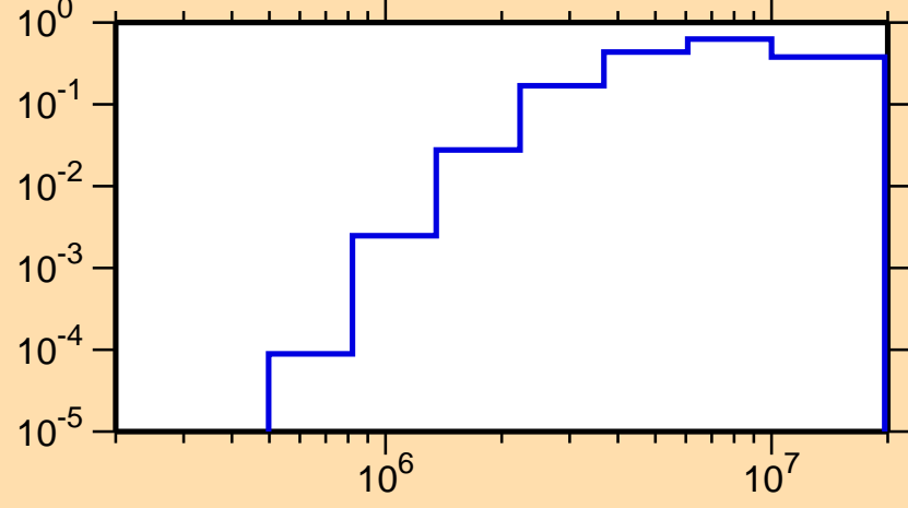
\sigma vs. E for ^{58}\text{Ni}(n,p)
