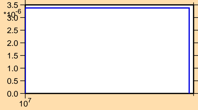
\sigma vs. E for ^{58}\text{Ni}(n,pd)
