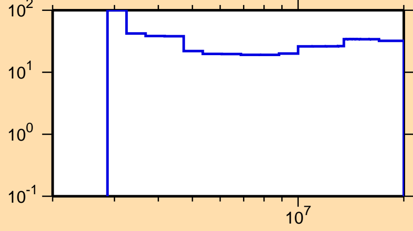
\Delta\sigma/\sigma vs. E for ^{59}\text{Ni}(n,n\text{cont.})
