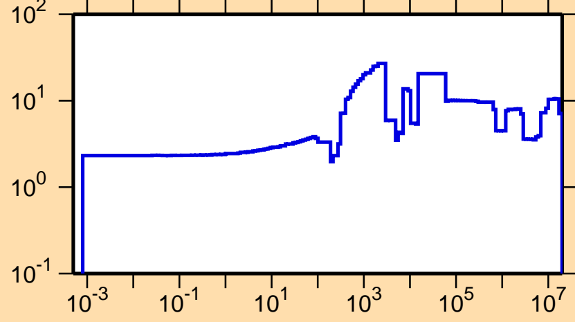
\Delta\sigma/\sigma vs. E for ^{59}\text{Ni}(n,\text{tot.})
