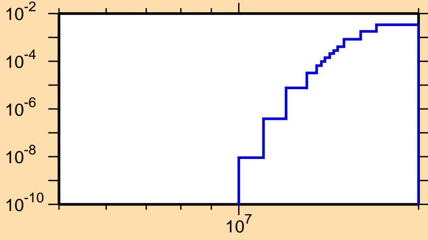
\sigma vs. E for ^{59}\text{Ni}(n,p\alpha)
