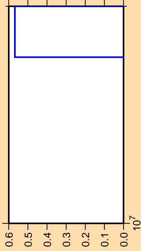
\Delta\sigma/\sigma vs. E for ^{59}\text{Ni}(\text{mt117})
