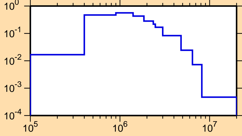
\sigma vs. E for ^{59}\text{Ni}(n,n_1)
