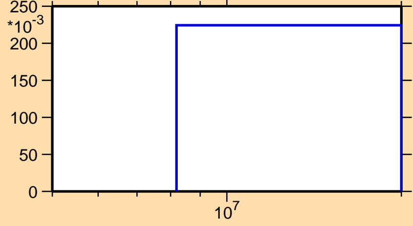
\sigma vs. E for ^{59}\text{Ni}(n,np)
