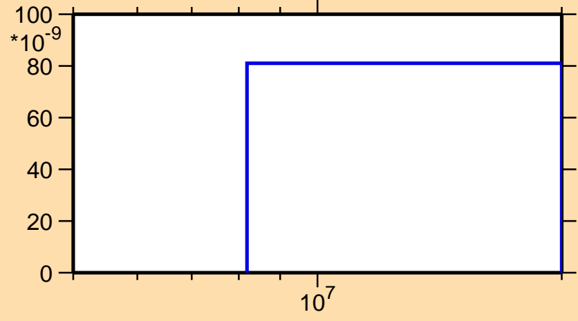
\sigma vs. E for ^{59}\text{Ni}(n,2np)
