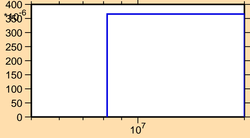
\sigma vs. E for ^{59}\text{Ni}(n,t)
