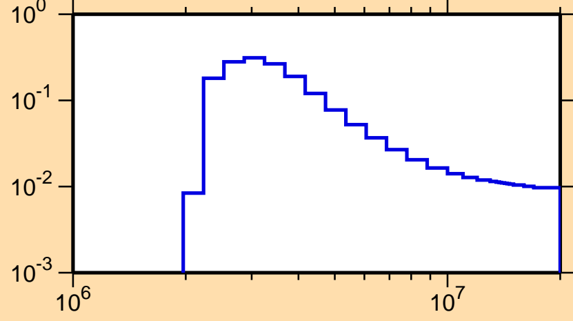
\sigma vs. E for ^{60}\text{Ni}(n,n_2)
