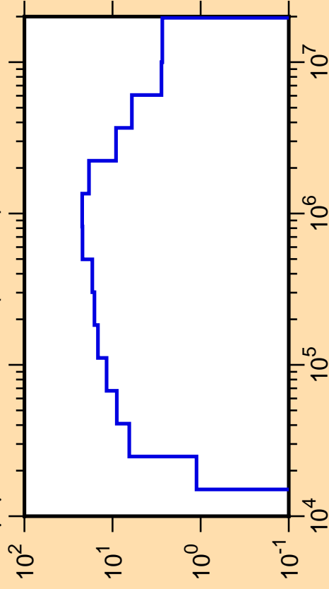
\Delta\mu/\mu vs. E for ^{60}\text{Ni}(\text{mt251})
