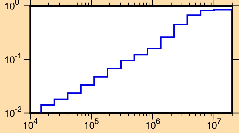
\mu vs. E for ^{60}\text{Ni}(\text{mt251})
