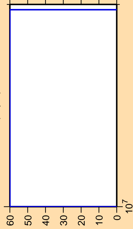
\Delta\sigma/\sigma vs. E for ^{60}\text{Ni}(n,pd)
