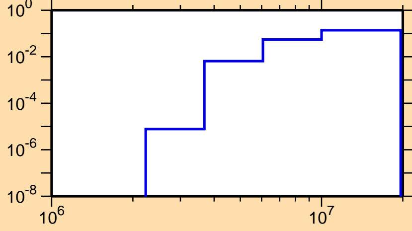
\sigma vs. E for ^{60}\text{Ni}(n,p)
