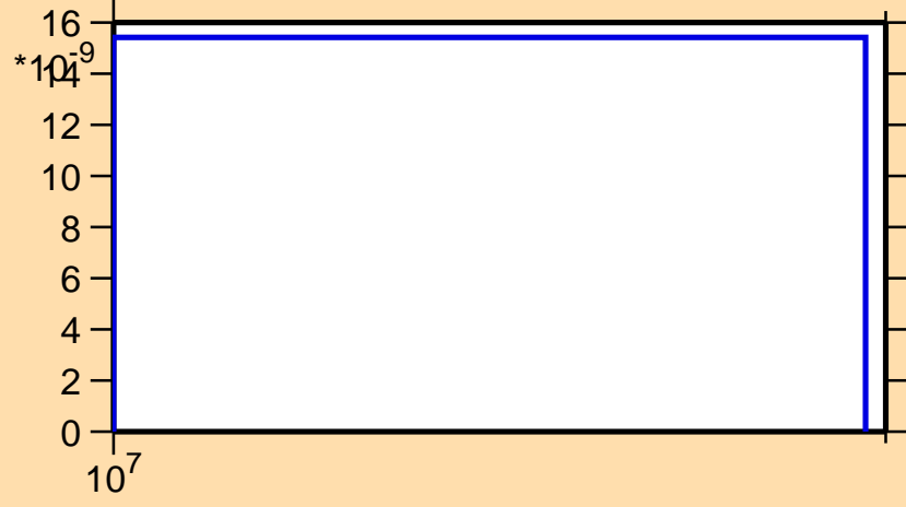
\sigma vs. E for ^{60}\text{Ni}(n,p\alpha)
