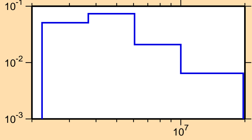
\sigma vs. E for ^{60}\text{Ni}(n,n_4)
