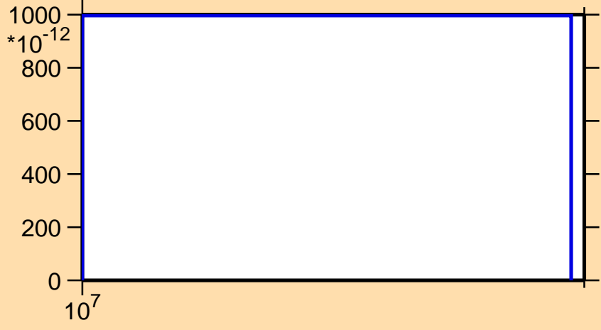
\sigma vs. E for ^{60}\text{Ni}(n,pd)
