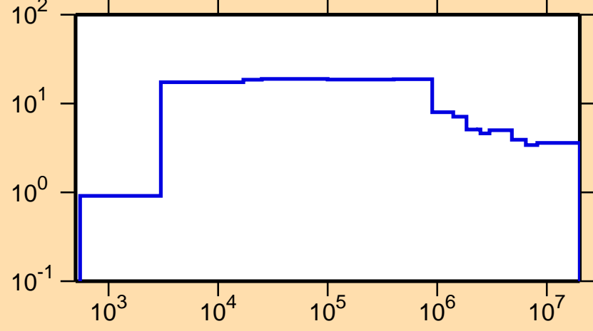
\Delta\sigma/\sigma vs. E for ^{60}\text{Ni}(n,\text{nonel.})
