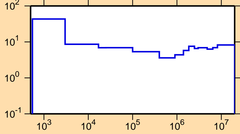
\Delta\sigma/\sigma vs. E for ^{60}\text{Ni}(n,\text{el.})
