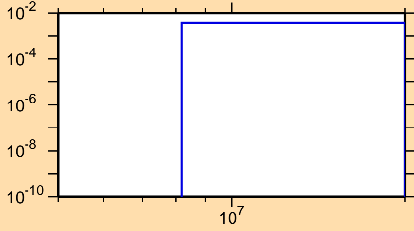
\sigma vs. E for ^{60}\text{Ni}(n,d)
