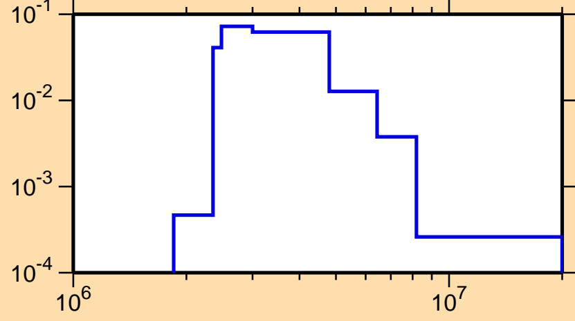
\sigma vs. E for ^{60}\text{Ni}(n,n_3)
