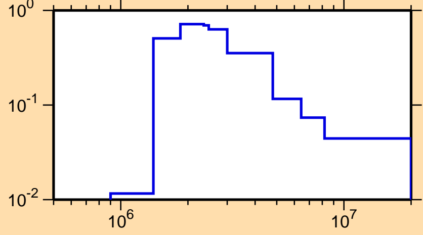
\sigma vs. E for ^{60}\text{Ni}(n,n_1)
