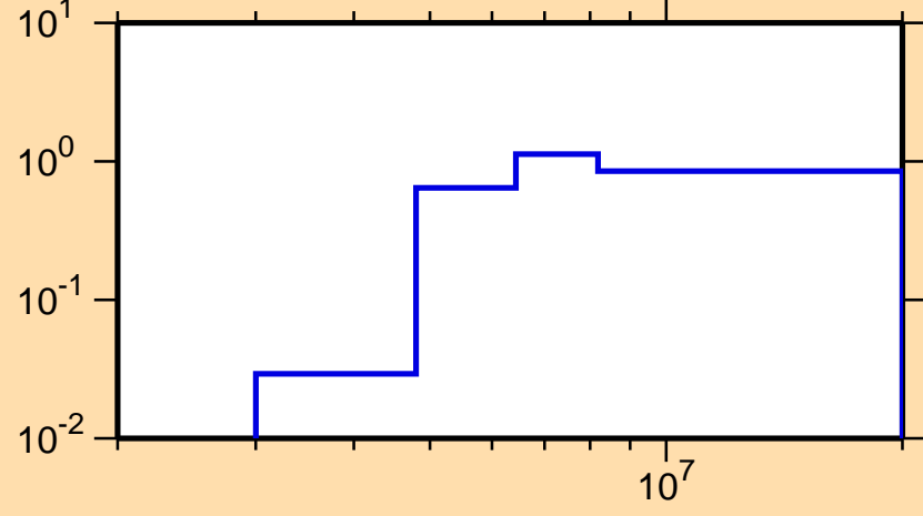
\sigma vs. E for ^{60}\text{Ni}(n,n\text{cont.})
