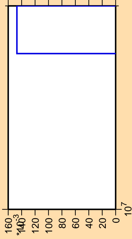
\Delta\sigma/\sigma vs. E for ^{61}\text{Ni}(n,nt)
