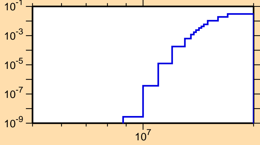
\sigma vs. E for ^{61}\text{Ni}(n,\alpha)
