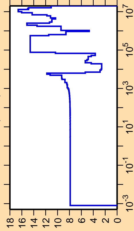
\Delta\sigma/\sigma vs. E for ^{61}\text{Ni}(n,\text{el.})
