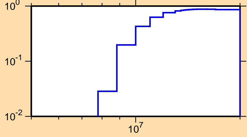
\sigma vs. E for ^{61}\text{Ni}(n,2n)
