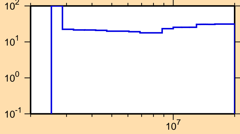
\Delta\sigma/\sigma vs. E for ^{61}\text{Ni}(n,n\text{cont.})
