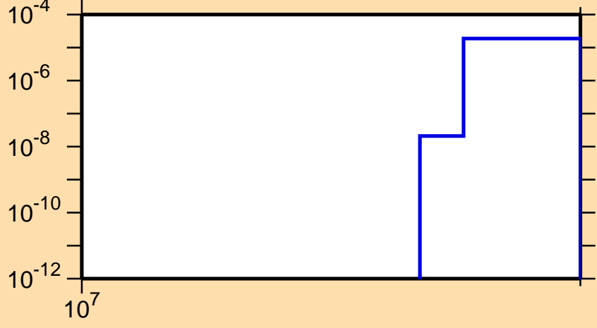
\sigma vs. E for ^{61}\text{Ni}(n,\text{nd})
