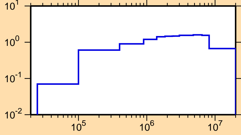
\sigma vs. E for ^{61}\text{Ni}(n,\text{inel.})
