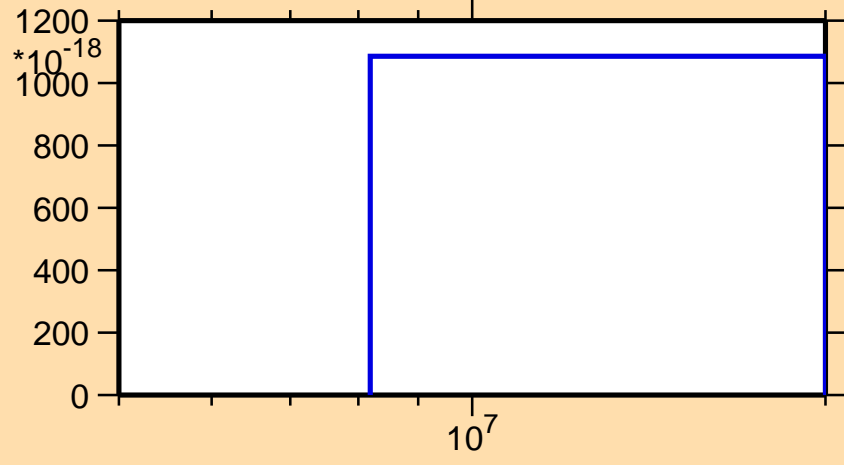
\sigma vs. E for ^{61}\text{Ni}(n,nt)
