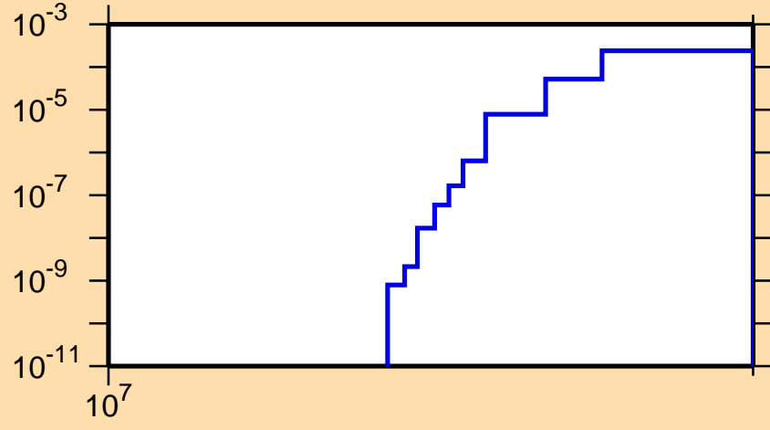
\sigma vs. E for ^{62}\text{Ni}(n,t)
