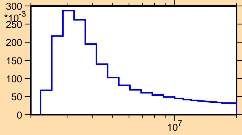
\sigma vs. E for ^{62}\text{Ni}(n,n_3)
