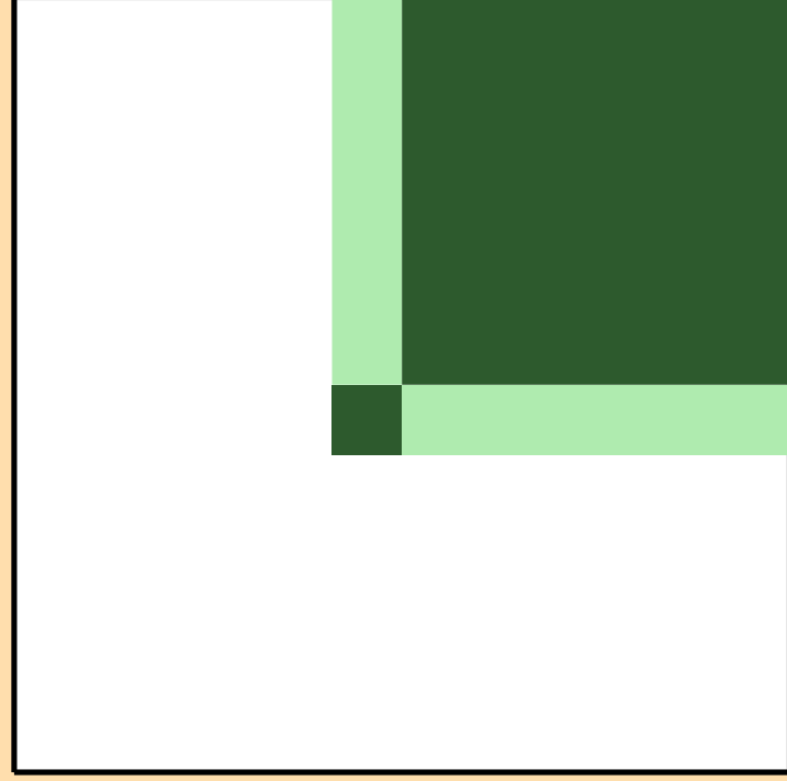
\sigma vs. E for ^{62}\text{Ni}(n,d)
