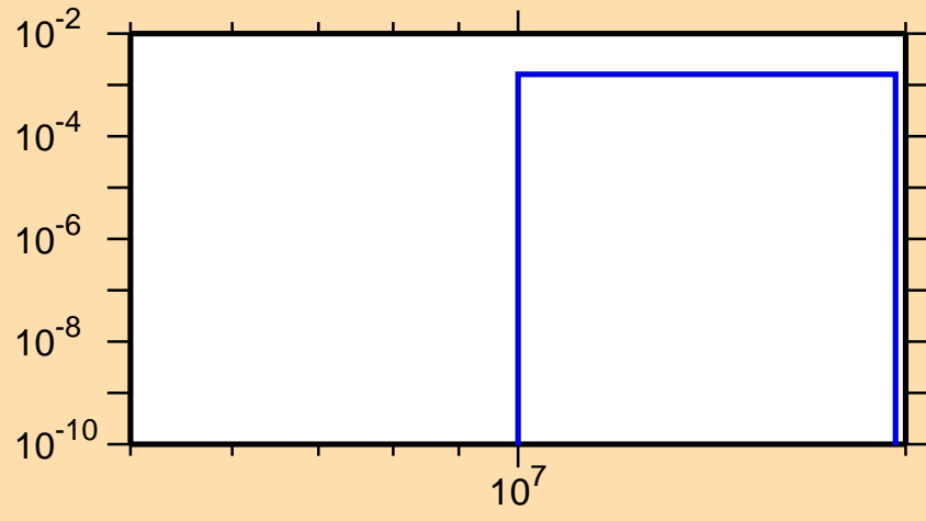
\sigma vs. E for ^{62}\text{Ni}(n,d)
