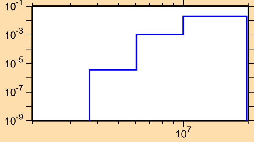
\sigma vs. E for ^{62}\text{Ni}(n,\alpha)
