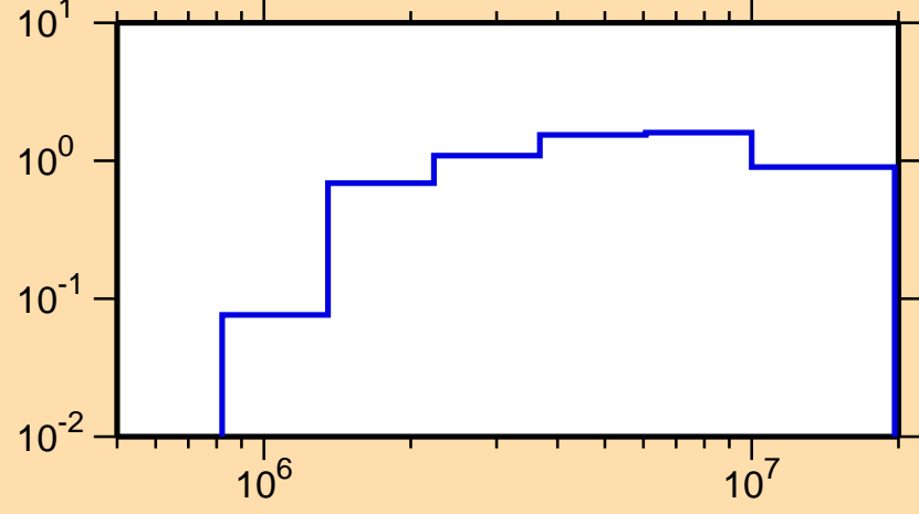
\sigma vs. E for ^{62}\text{Ni}(n,\text{inel.})
