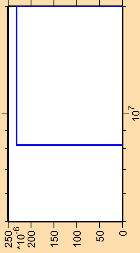
\Delta\sigma/\sigma vs. E for ^{62}\text{Ni}(n,nt)
