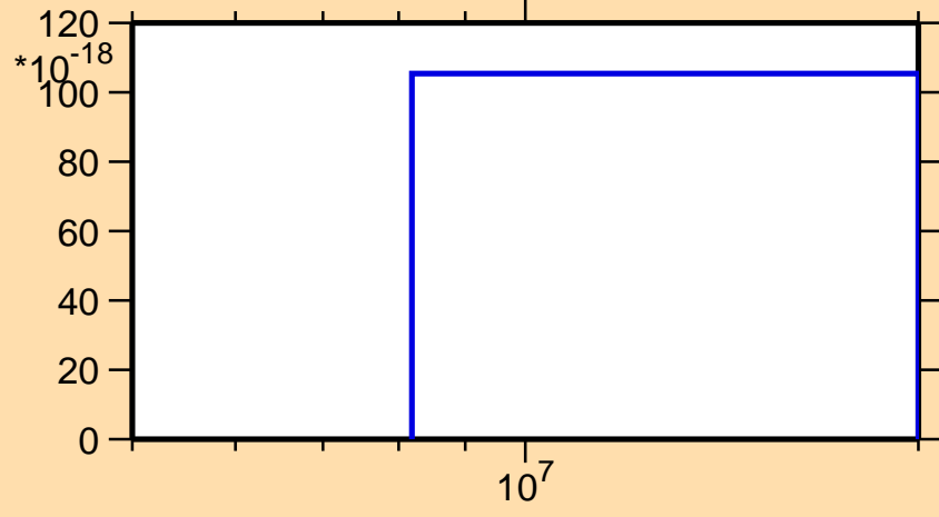
\sigma vs. E for ^{62}\text{Ni}(n,nt)
