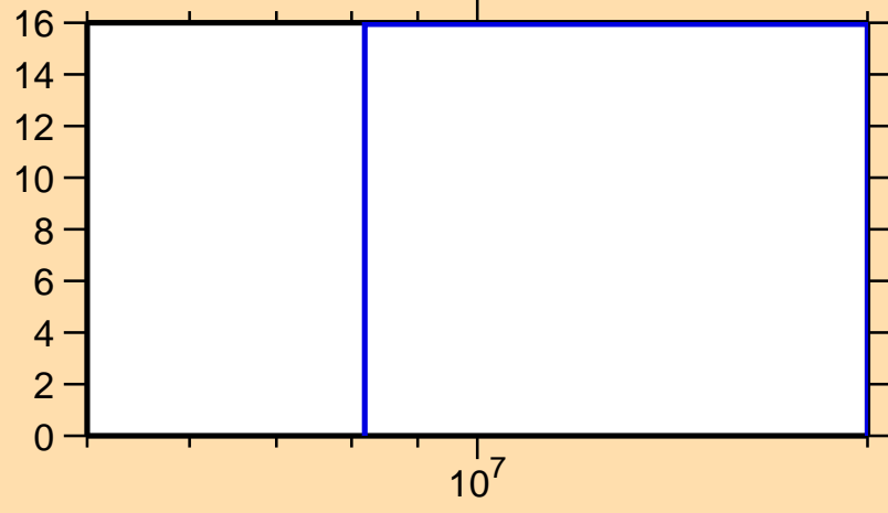
\Delta\sigma/\sigma vs. E for ^{62}\text{Ni}(n,2n)
