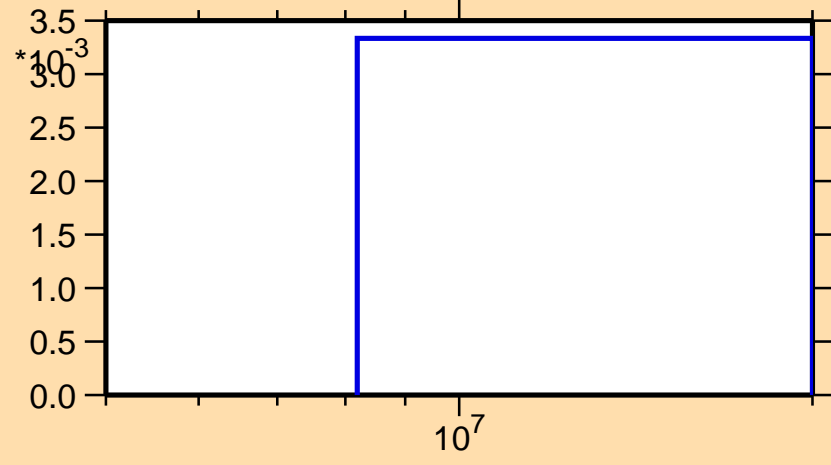
\sigma vs. E for ^{62}\text{Ni}(n,np)
