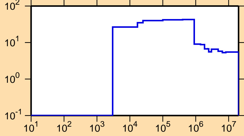
\Delta\sigma/\sigma vs. E for ^{62}\text{Ni}(n,\text{nonel.})
