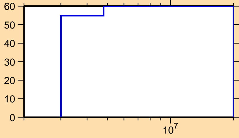
\Delta\sigma/\sigma vs. E for ^{62}\text{Ni}(n,\gamma)
