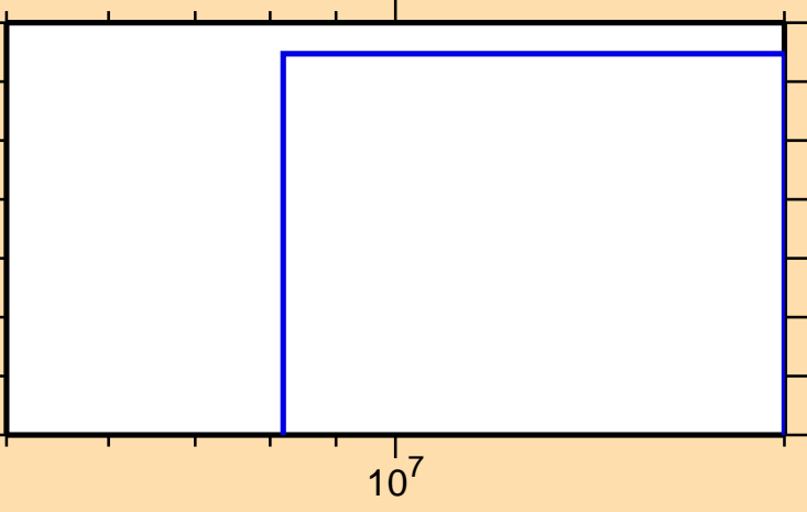
\sigma vs. E for ^{62}\text{Ni}(n,d)
