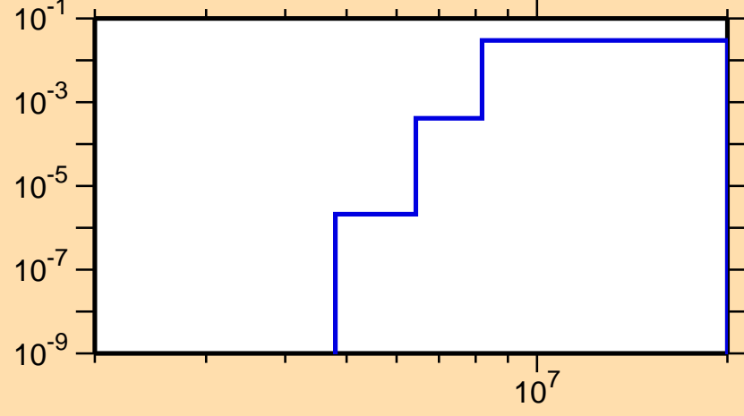
\sigma vs. E for ^{62}\text{Ni}(n,p)
