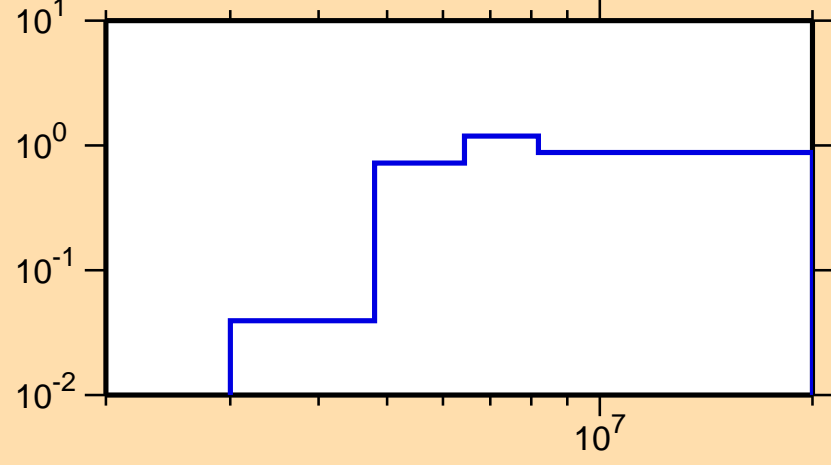
\sigma vs. E for ^{62}\text{Ni}(n,n\text{cont.})
