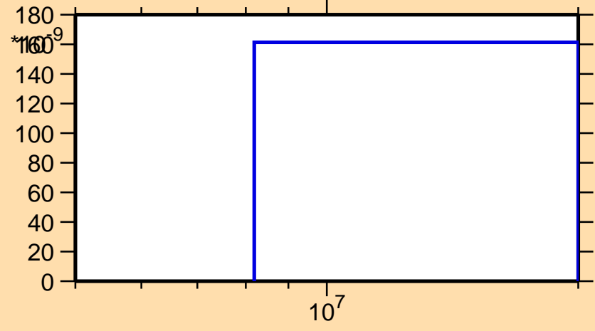
\sigma vs. E for ^{62}\text{Ni}(n,3n)
