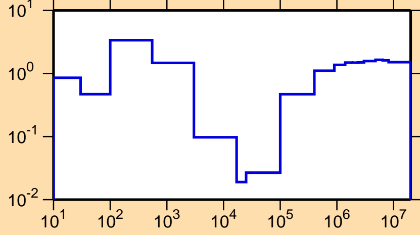
\sigma vs. E for ^{63}\text{Ni}(n,\text{nonel.})
