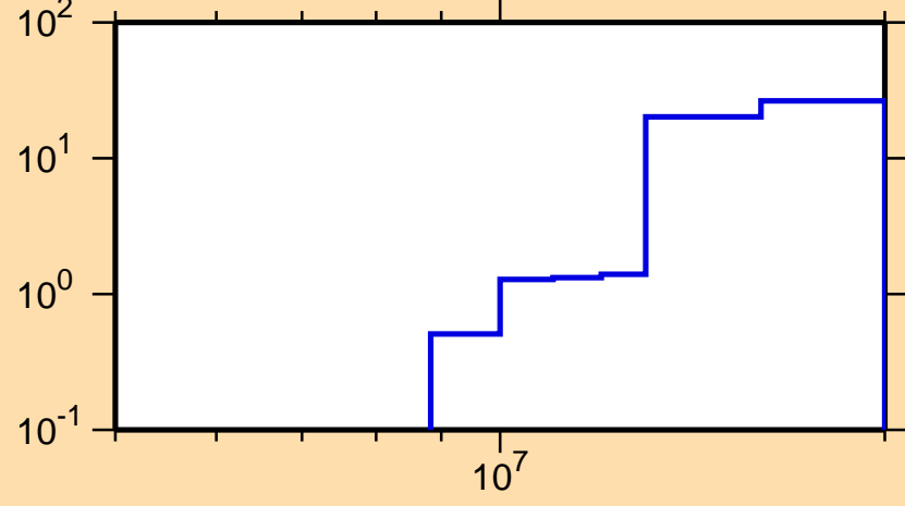
\Delta\sigma/\sigma vs. E for ^{64}\text{Ni}(n,\text{inel.})
