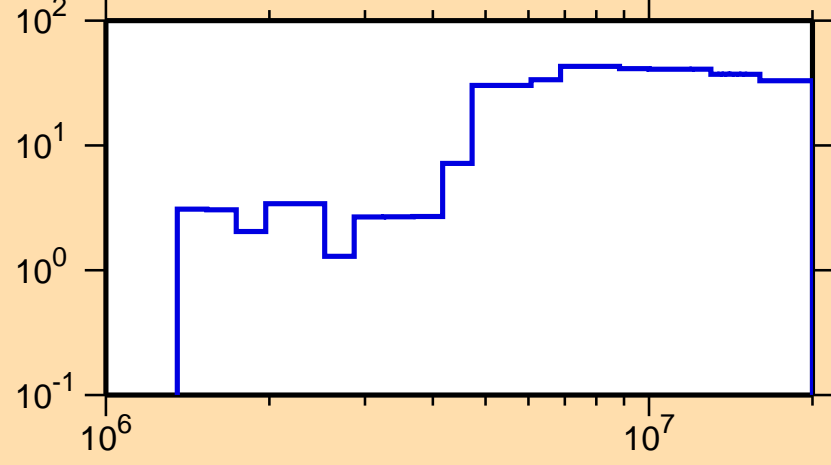
\Delta\sigma/\sigma vs. E for ^{64}\text{Ni}(n,n_1)
