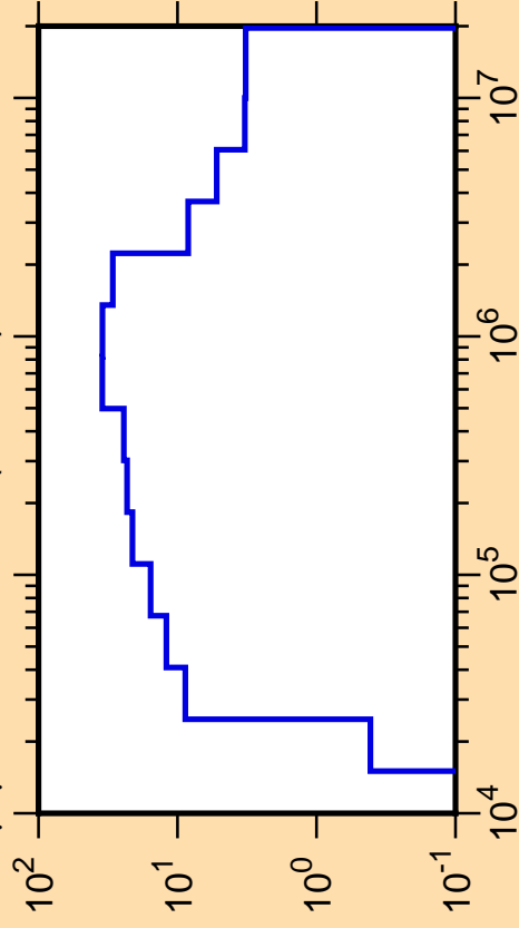
\Delta\mu/\mu vs. E for ^{64}\text{Ni}(\text{mt251})
