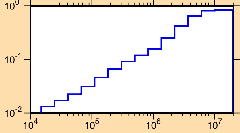
\mu vs. E for ^{64}\text{Ni}(\text{mt251})
