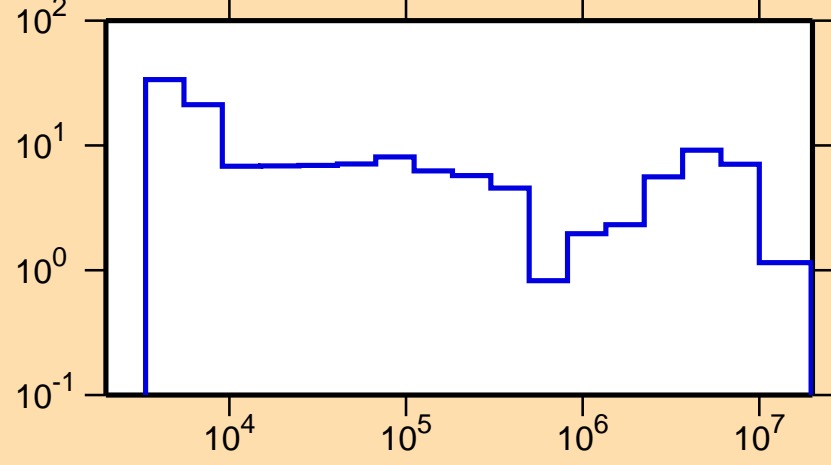
\Delta\sigma/\sigma vs. E for ^{64}\text{Ni}(n,\text{el.})
