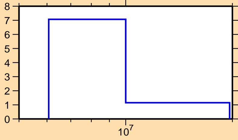
\Delta\sigma/\sigma vs. E for ^{64}\text{Ni}(n,el.)
