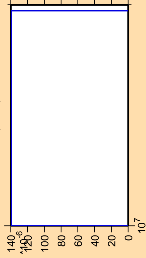
\Delta\sigma/\sigma vs. E for ^{64}\text{Ni}(n,\text{nd})
