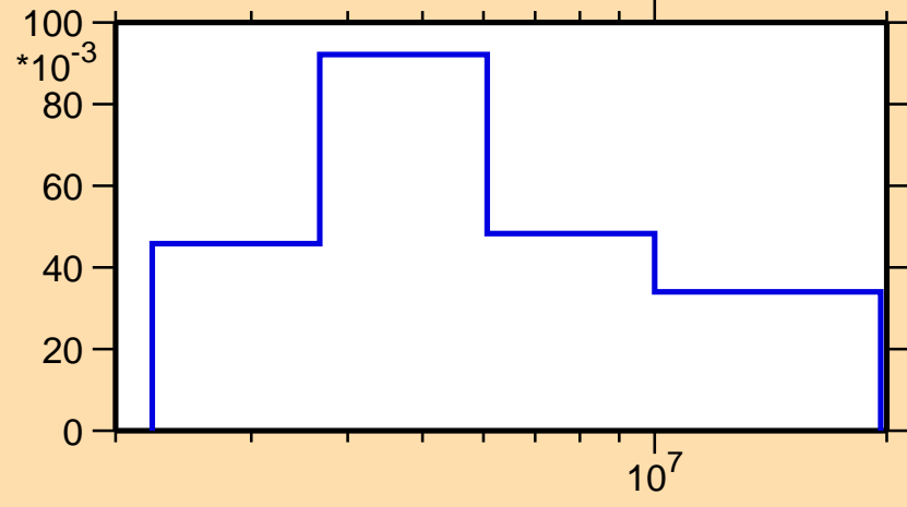
\sigma vs. E for ^{64}\text{Ni}(n,n_4)
