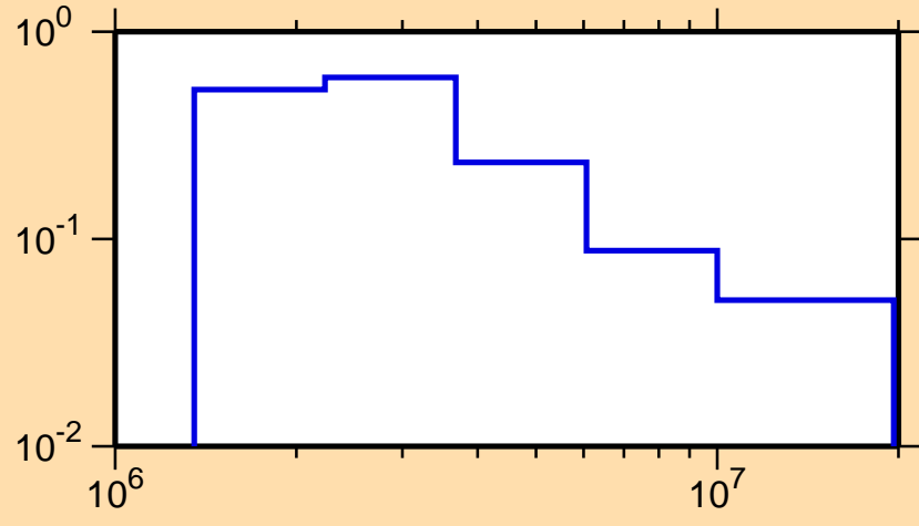
\sigma vs. E for ^{64}\text{Ni}(n,n_1)
