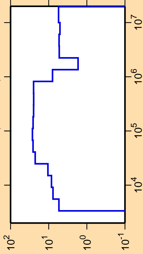
\Delta\sigma/\sigma vs. E for ^{64}\text{Ni}(n,\text{nonel.})
