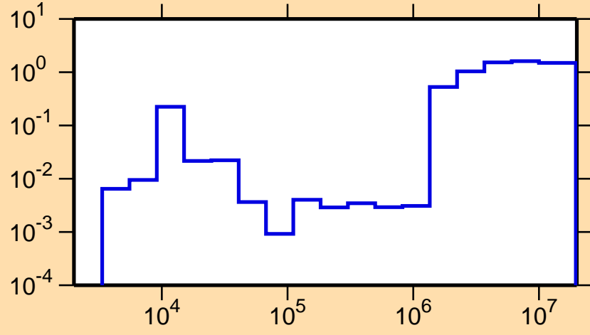
\sigma vs. E for ^{64}\text{Ni}(n,\text{nonel.})
