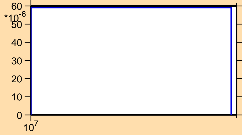
\sigma vs. E for ^{64}\text{Ni}(n,3n)
