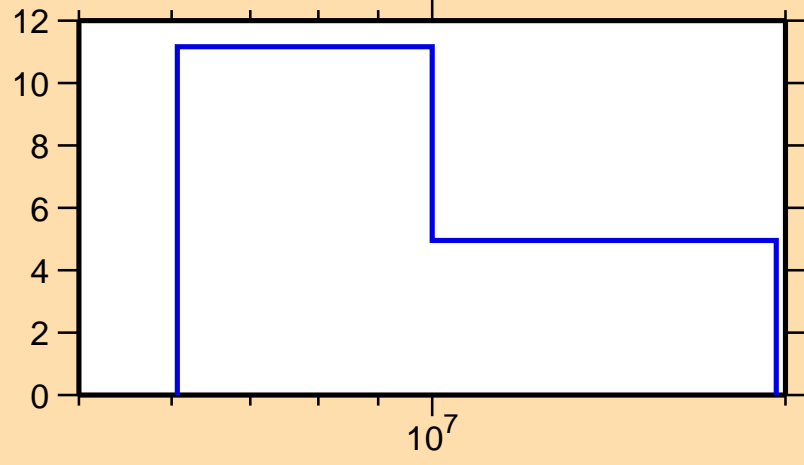
\Delta\sigma/\sigma vs. E for ^{64}\text{Ni}(n,ncont.)
