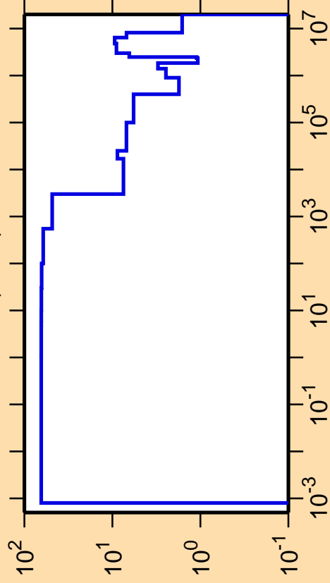
\Delta\sigma/\sigma vs. E for ^{64}\text{Ni}(n,\text{el.})
