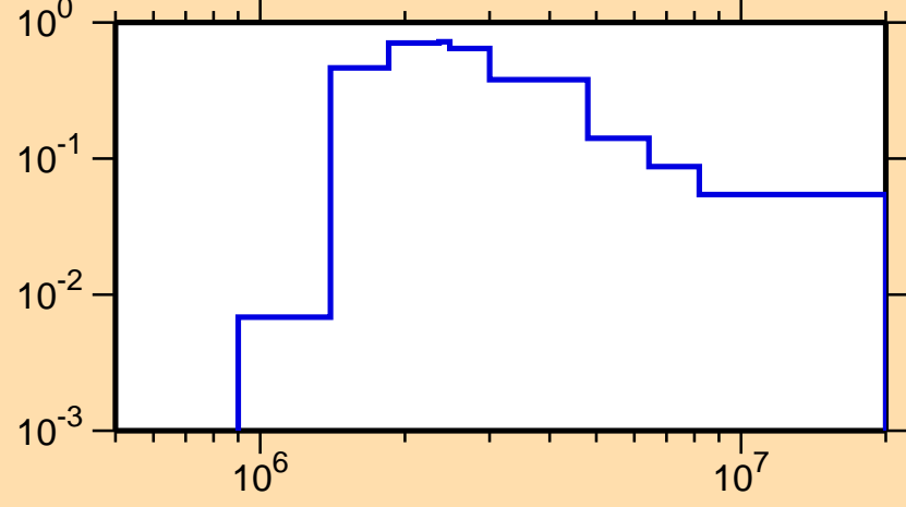
\sigma vs. E for ^{64}\text{Ni}(n,n_1)
