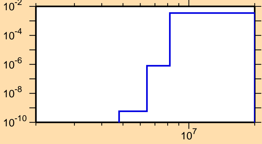
\sigma vs. E for ^{64}\text{Ni}(n,\alpha)
