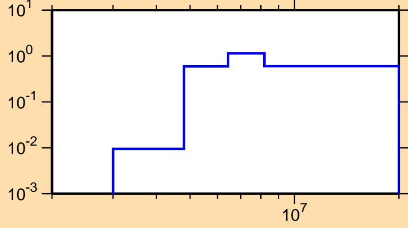
\sigma vs. E for ^{64}\text{Ni}(n,n\text{cont.})
