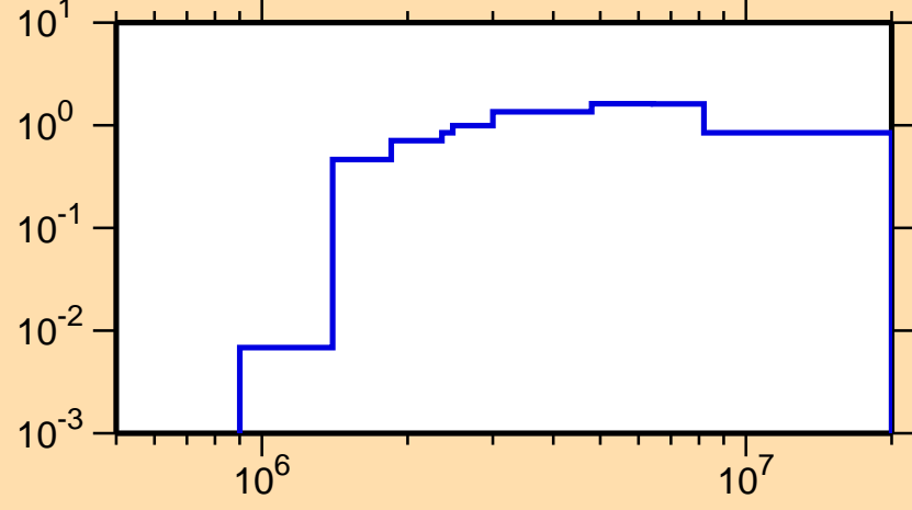
\sigma vs. E for ^{64}\text{Ni}(n,\text{inel.})
