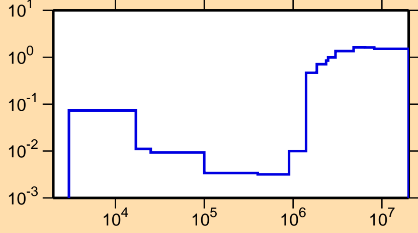
\sigma vs. E for ^{64}\text{Ni}(n,\text{nonel.})
