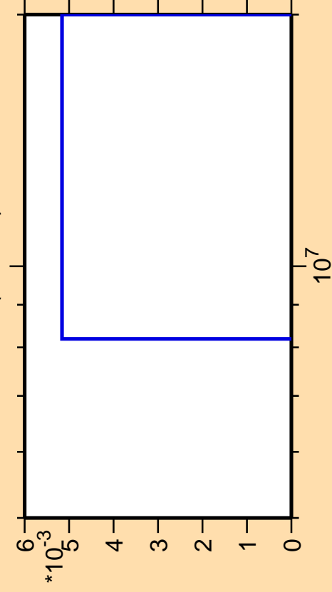
\Delta\sigma/\sigma vs. E for ^{64}\text{Ni}(n,\text{He}3)
