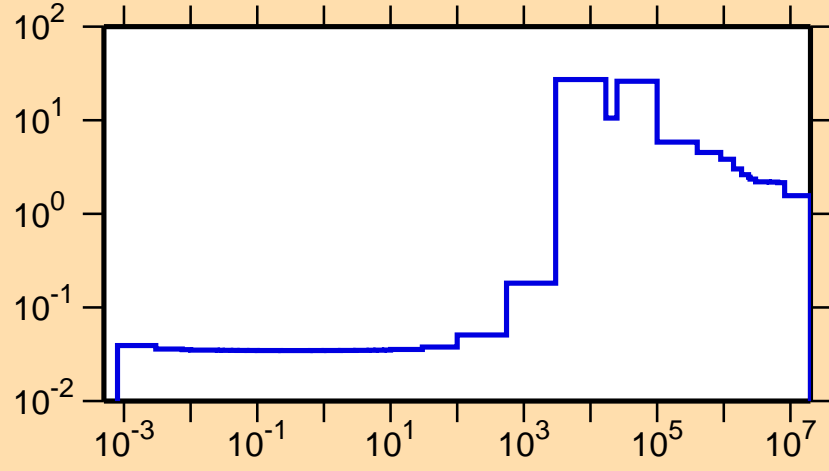
\sigma vs. E for ^{64}\text{Ni}(n,\text{el.})
