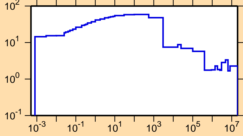
\Delta\sigma/\sigma vs. E for ^{64}\text{Ni}(n,\text{tot.})
