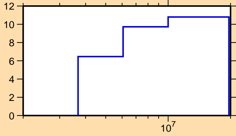
\Delta\sigma/\sigma vs. E for ^{65}\text{Ni}(n,el.)
