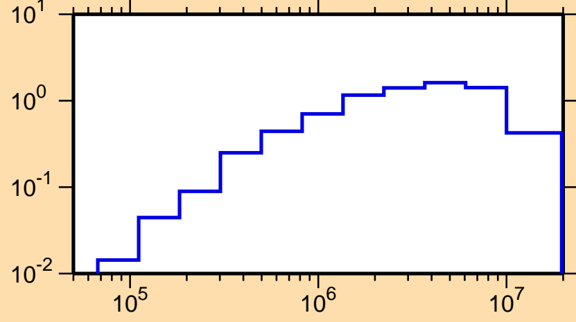
\sigma vs. E for ^{65}\text{Ni}(n,\text{inel.})
