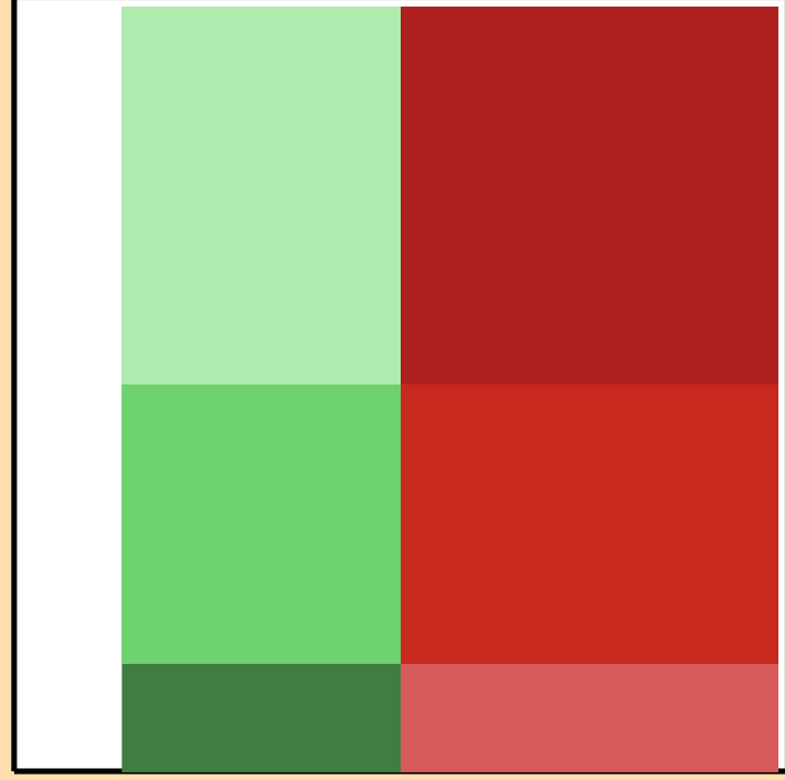
\Delta\sigma/\sigma vs. E for ^{65}\text{Ni}(n,2n)
