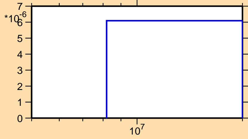
\sigma vs. E for ^{65}\text{Ni}(n,t)
