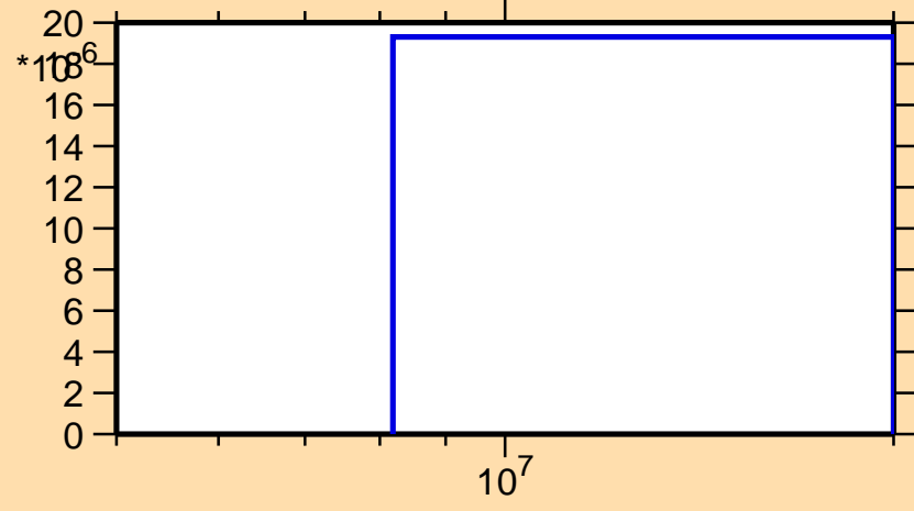
\sigma vs. E for ^{65}\text{Ni}(n,\alpha)
