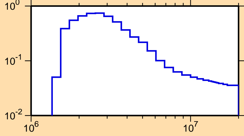
\sigma vs. E for ^{66}\text{Ni}(n,n_1)
