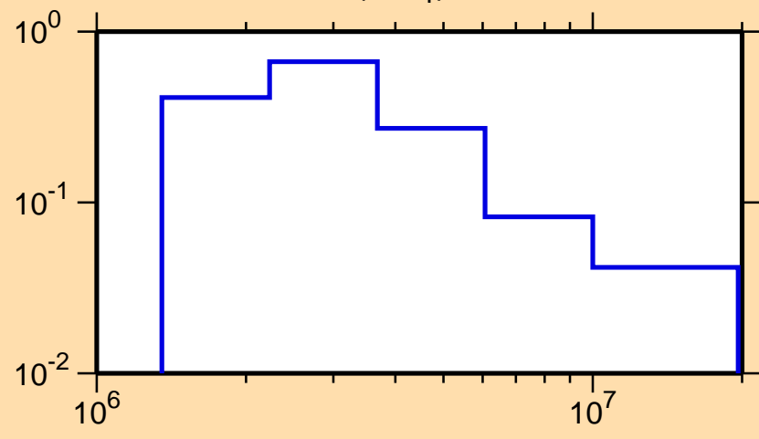
\sigma vs. E for ^{66}\text{Ni}(n,n_1)
