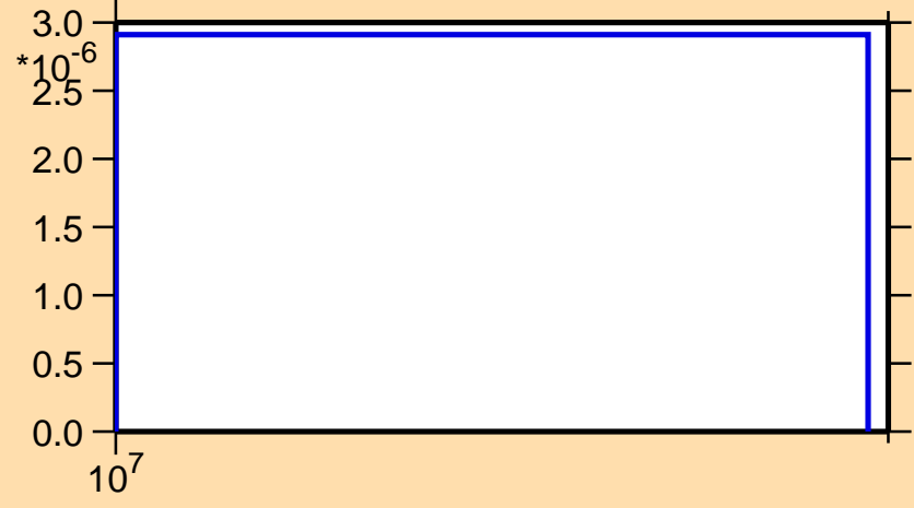
\sigma vs. E for ^{66}\text{Ni}(n,np)
