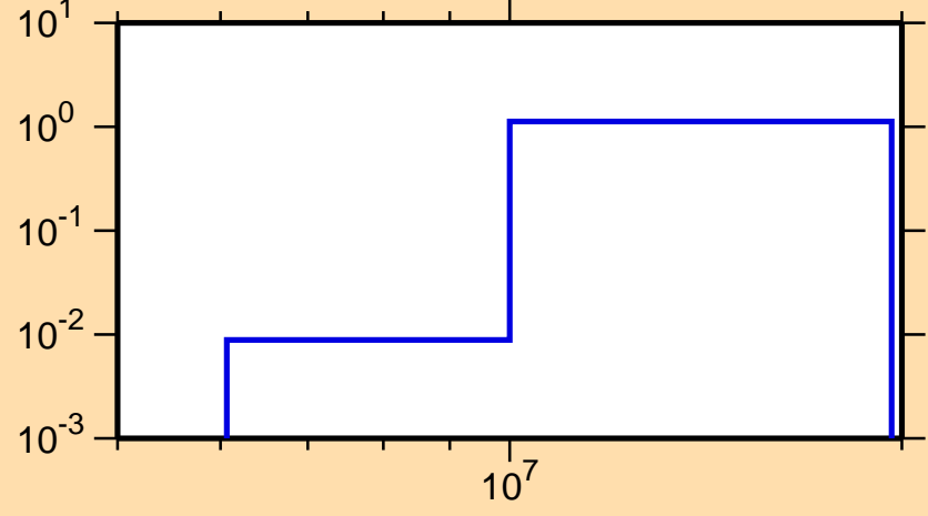
\sigma vs. E for ^{66}\text{Ni}(n,2n)
