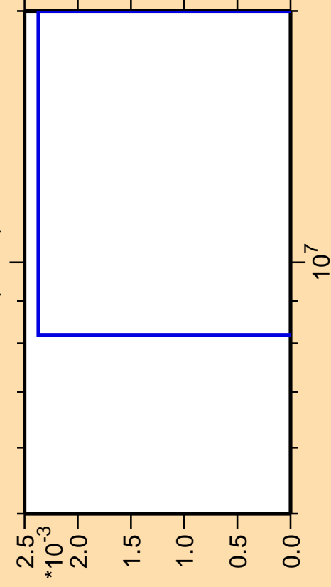
\Delta\sigma/\sigma vs. E for ^{66}\text{Ni}(n,\text{nd})
