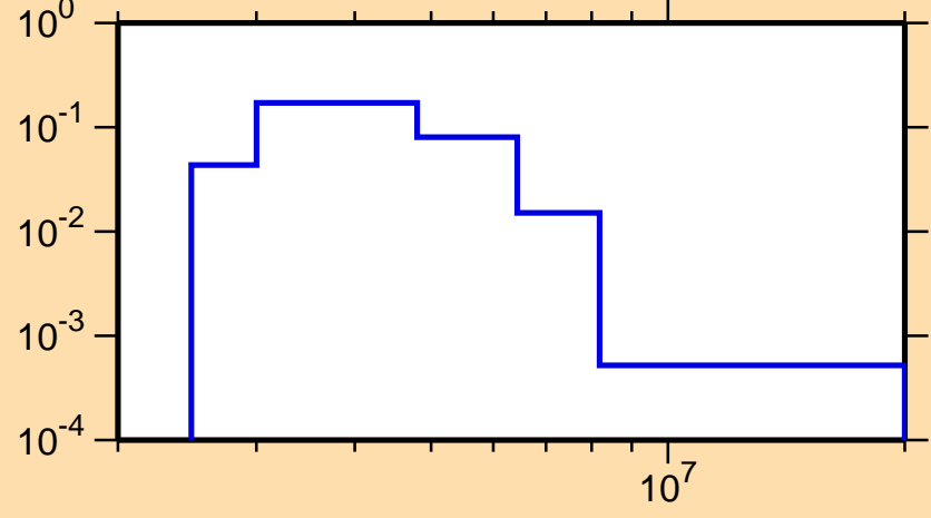
\sigma vs. E for ^{66}\text{Ni}(n,n_4)
