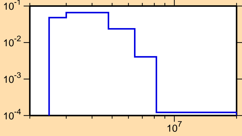
\sigma vs. E for ^{66}\text{Ni}(n,n_2)
