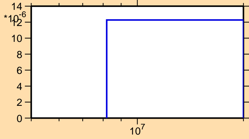
\sigma vs. E for ^{66}\text{Ni}(n,d)
