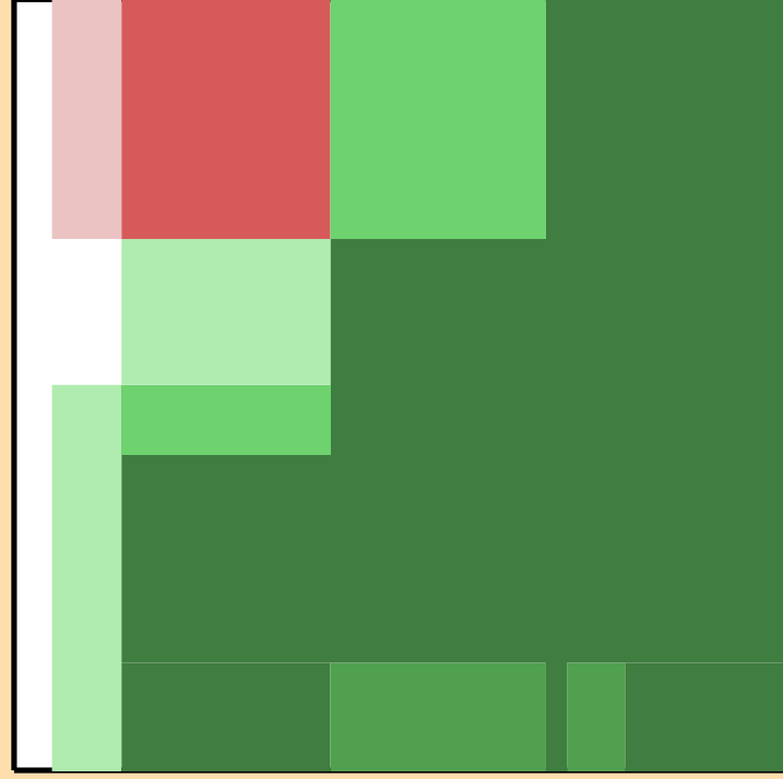
\Delta\sigma/\sigma vs. E for ^{68}\text{Ni}(n,n\text{cont.})
