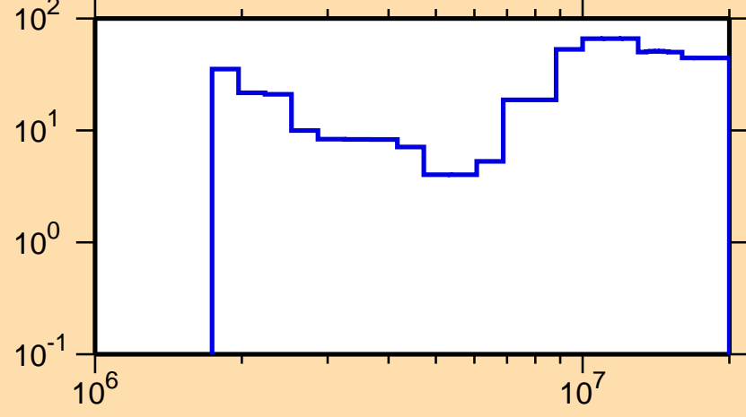
\Delta\sigma/\sigma vs. E for ^{68}\text{Ni}(n,\text{inel.})
