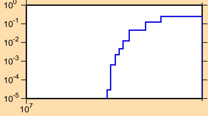
\sigma vs. E for ^{68}\text{Ni}(n,3n)
