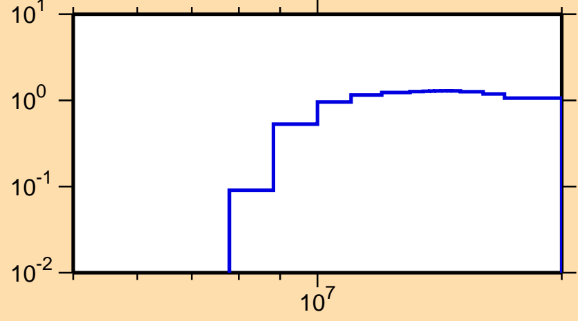
\sigma vs. E for ^{68}\text{Ni}(n,2n)
