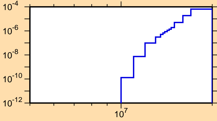
\sigma vs. E for ^{68}\text{Ni}(n,\alpha)
