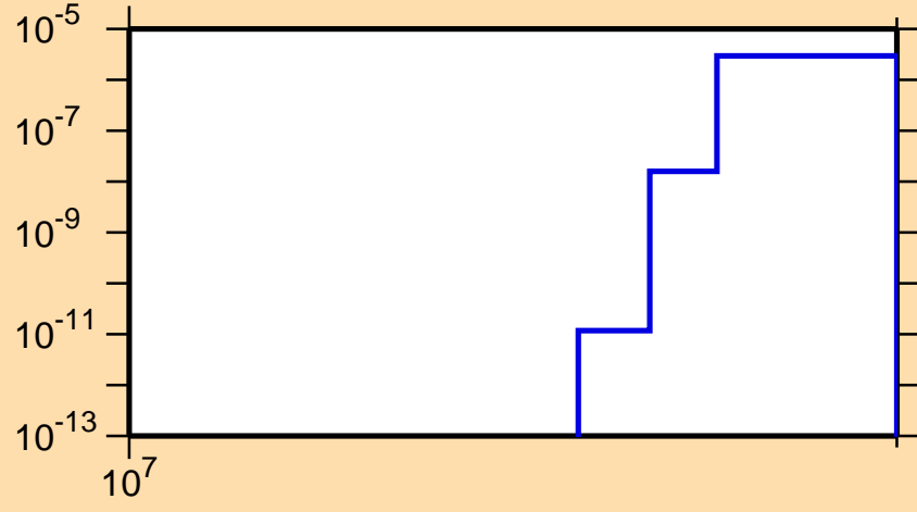
\sigma vs. E for ^{68}\text{Ni}(n,t)
