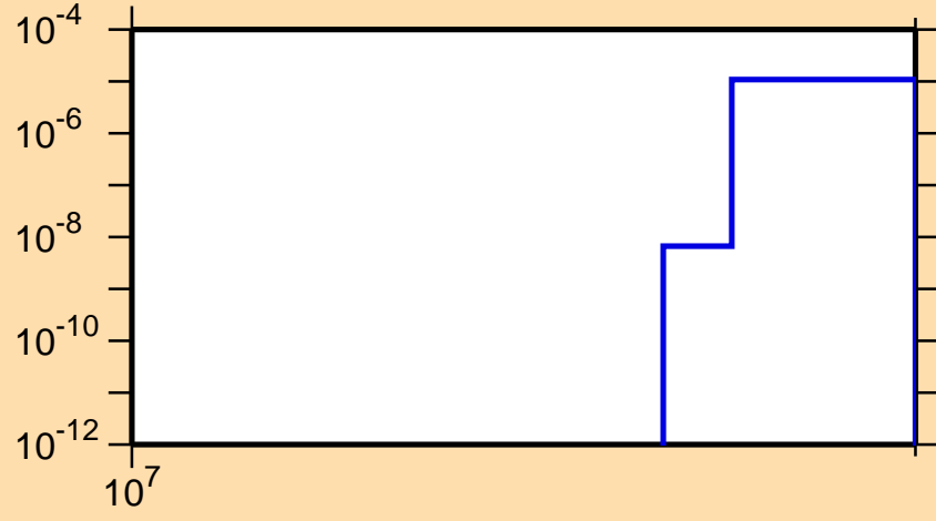
\sigma vs. E for ^{68}\text{Ni}(n,np)
