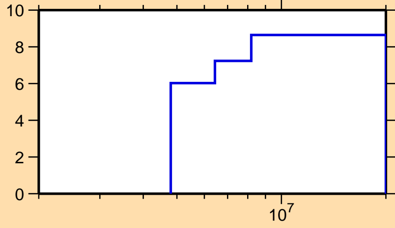
\Delta\sigma/\sigma vs. E for ^{68}\text{Ni}(n,n\text{onel.})
