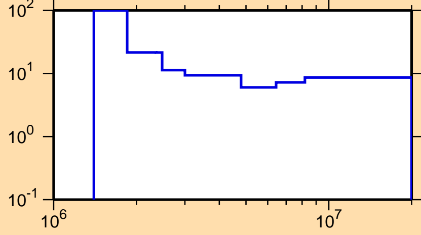
\Delta\sigma/\sigma vs. E for ^{68}\text{Ni}(n,\text{nonel.})
