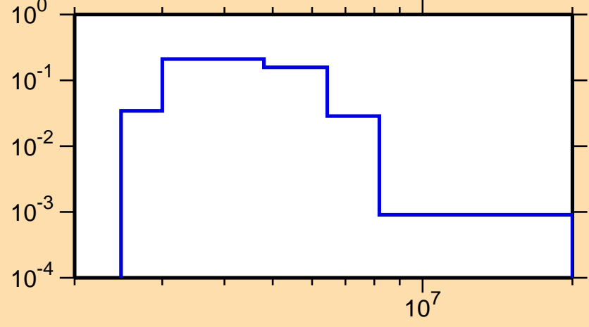
\sigma vs. E for ^{68}\text{Ni}(n,n_4)
