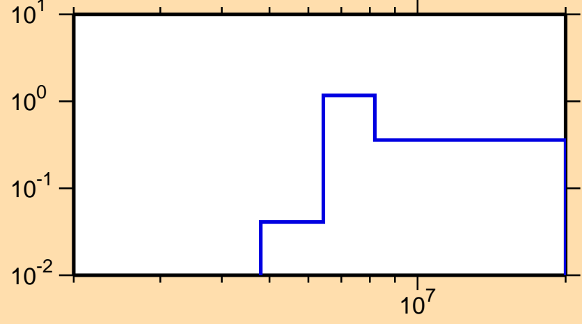
\sigma vs. E for ^{68}\text{Ni}(n,n\text{cont.})
