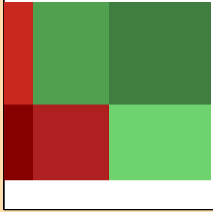
\Delta\sigma/\sigma vs. E for ^{69}\text{Ni}(n,n_1)
