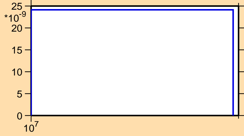
\sigma vs. E for ^{69}\text{Ni}(n,n\alpha)
