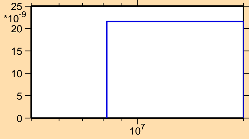
\sigma vs. E for ^{69}\text{Ni}(n,\alpha)
