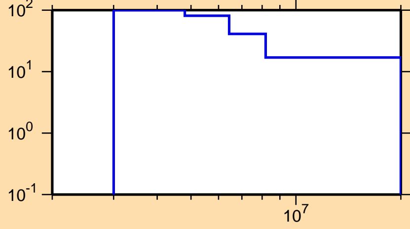
\Delta\sigma/\sigma vs. E for ^{69}\text{Ni}(n,2n)
