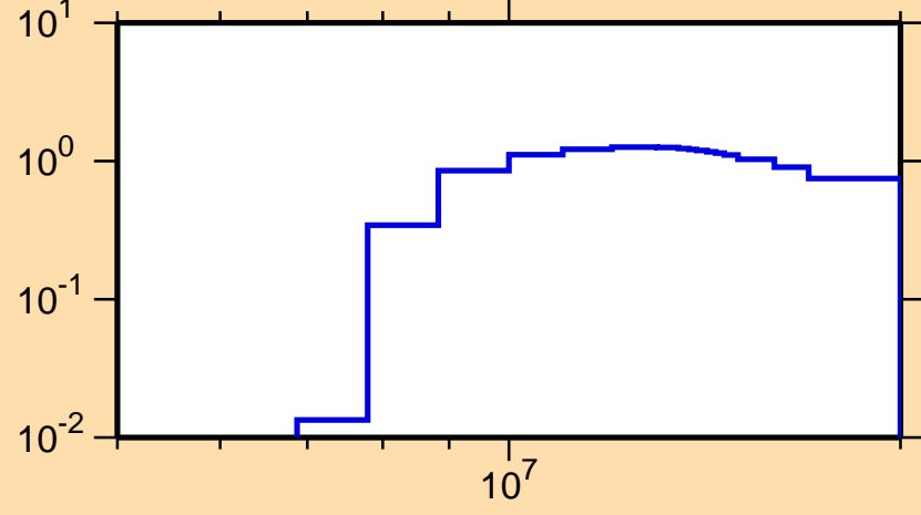
\sigma vs. E for ^{70}\text{Ni}(n,2n)
