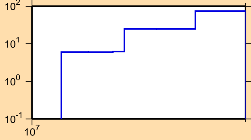
\Delta\sigma/\sigma vs. E for ^{70}\text{Ni}(n,2n)
