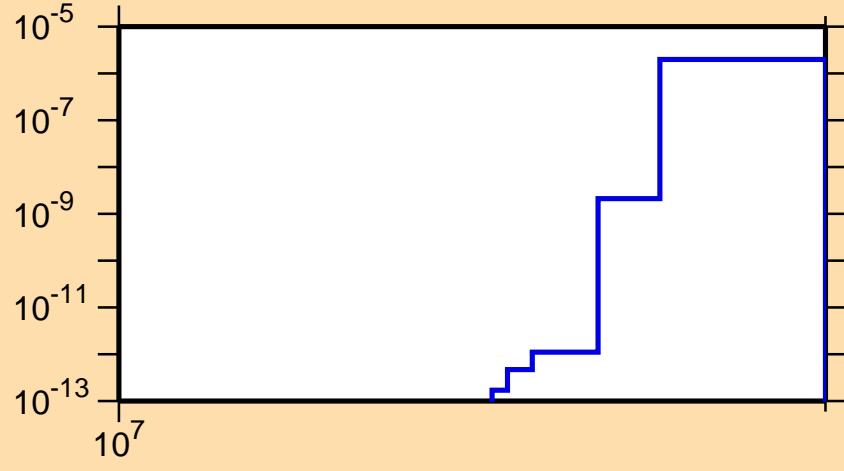
\sigma vs. E for ^{70}\text{Ni}(n,t)
