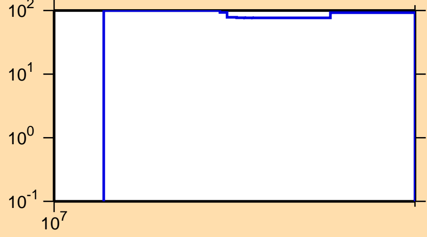
\Delta\sigma/\sigma vs. E for ^{70}\text{Ni}(n,p)
