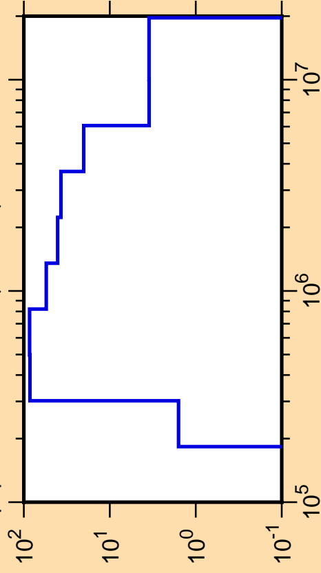
\Delta\mu/\mu vs. E for ^{70}\text{Ni}(\text{mt251})
