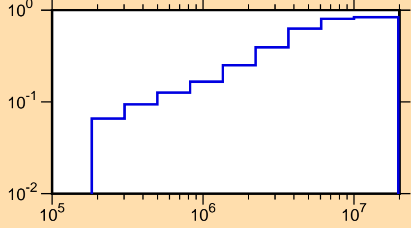
\mu vs. E for ^{70}\text{Ni}(\text{mt251})
