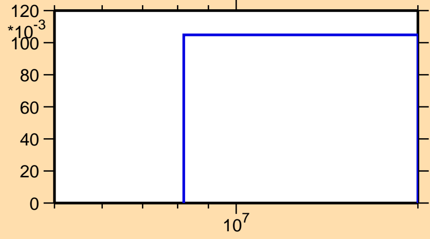
\sigma vs. E for ^{70}\text{Ni}(n,3n)
