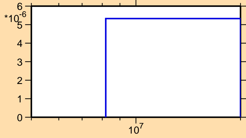
\sigma vs. E for ^{70}\text{Ni}(n,p)
