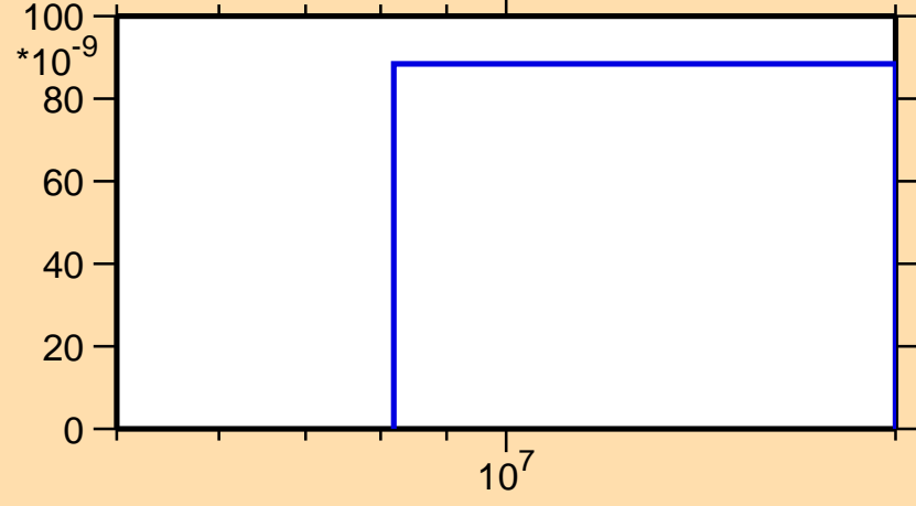
\sigma vs. E for ^{70}\text{Ni}(n,\alpha)
