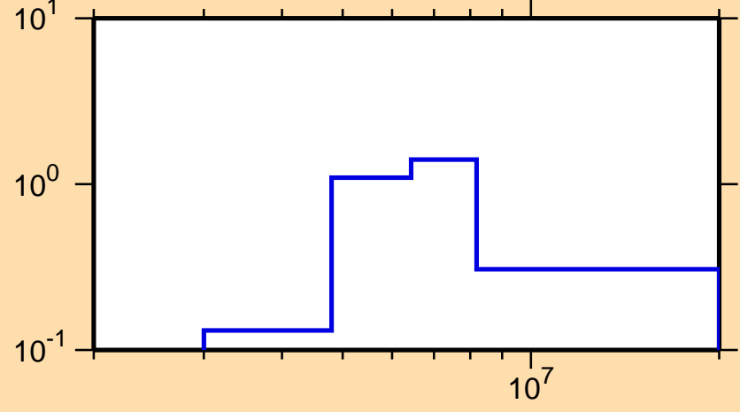
\sigma vs. E for ^{70}\text{Ni}(n,n\text{cont.})
