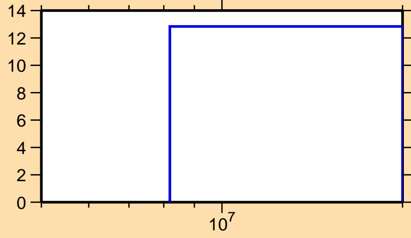
\Delta\sigma/\sigma vs. E for ^{70}\text{Ni}(n,el.)
