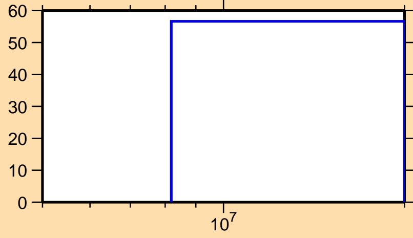
\Delta\sigma/\sigma vs. E for ^{70}\text{Ni}(n,ncont.)
