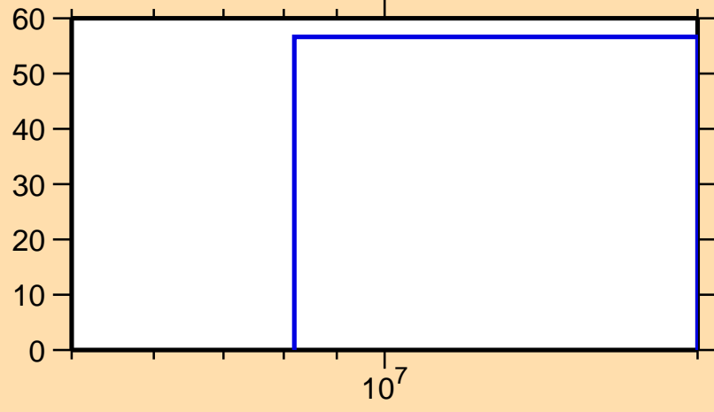
\Delta\sigma/\sigma vs. E for ^{70}\text{Ni}(n,n\text{cont.})
