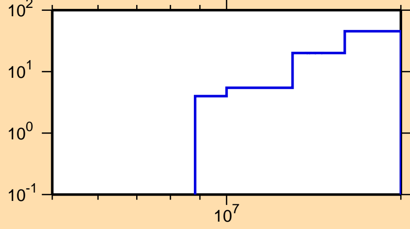
\Delta\sigma/\sigma vs. E for ^{71}\text{Ni}(n,2n)
