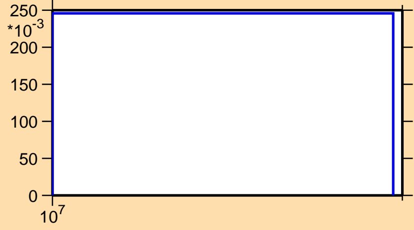
\sigma vs. E for ^{71}\text{Ni}(n,3n)
