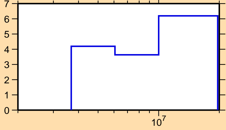
\Delta\sigma/\sigma vs. E for ^{71}\text{Ni}(n,\text{nonel.})
