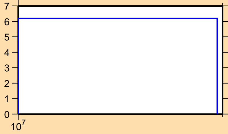
\Delta\sigma/\sigma vs. E for ^{71}\text{Ni}(n,\text{nonel.})
