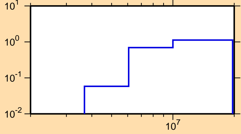
\sigma vs. E for ^{71}\text{Ni}(n,2n)
