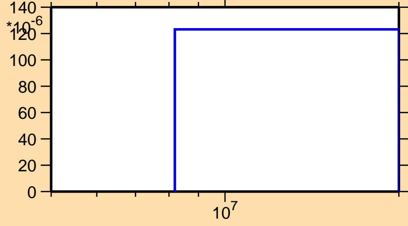
\sigma vs. E for ^{71}\text{Ni}(n,p)
